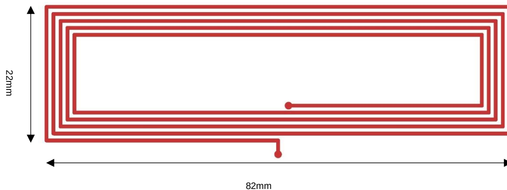
ANT2- NFC Antenna Copper Patterns
