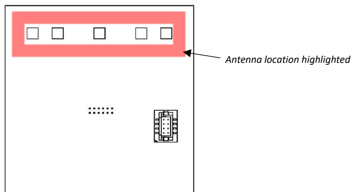
ANT2- NFC Antenna Location
