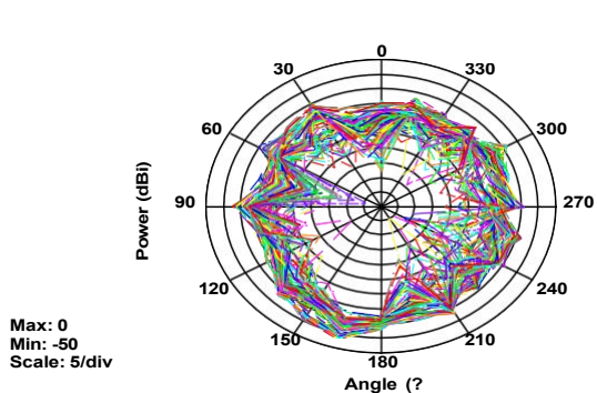
Horizontally Polarized XZ plane
