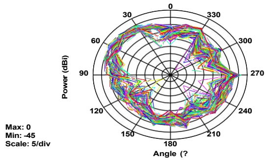
Vertical Polarization XY plane
