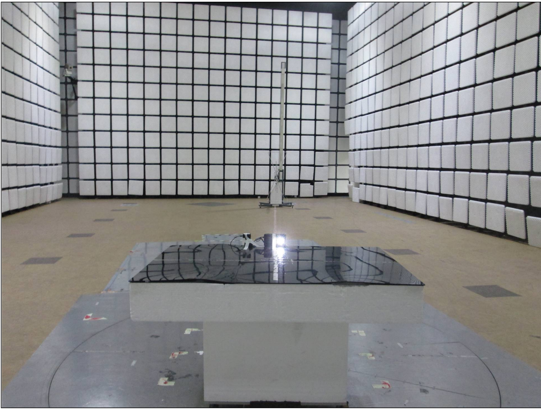
RE(Below 1 GHz)_Front
