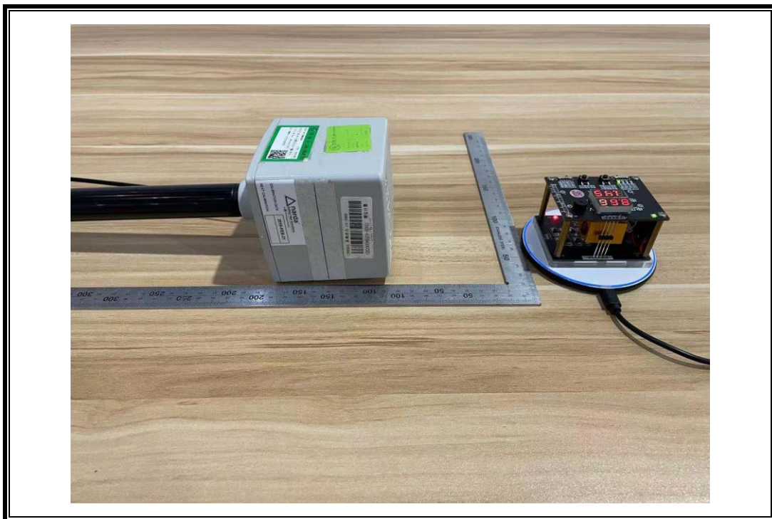
E-FILED AND H-FILED STRENGTH MEASUREMENT SETUP-C
