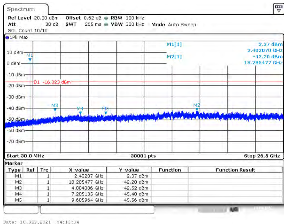
Tx. Spurious NVNT 1-DH1 2402MHz Ant1 Emission
