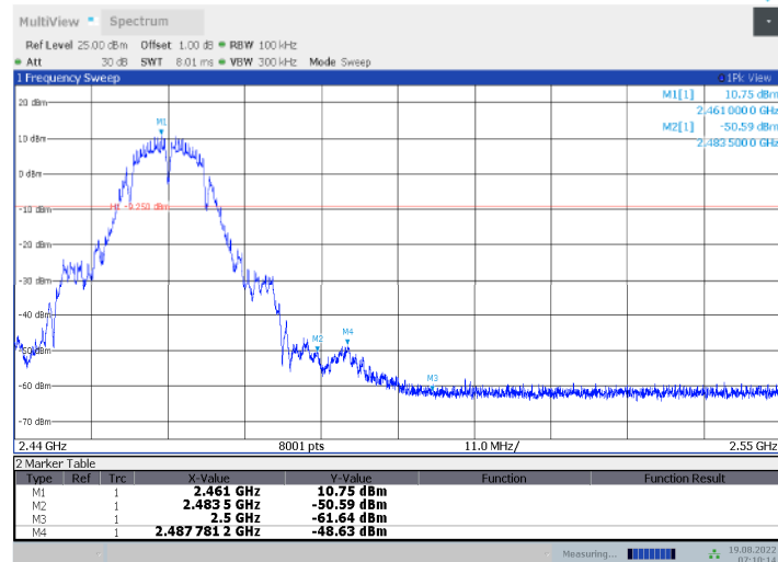
11B_Ant2_High_2462
