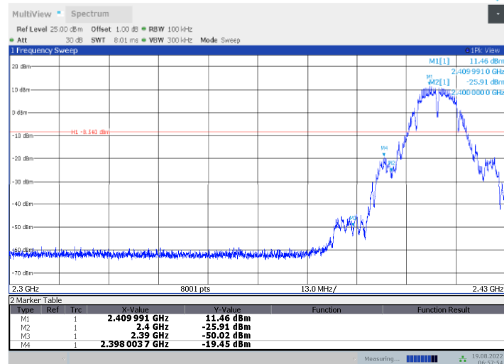
11B_Ant2_Low_2412
