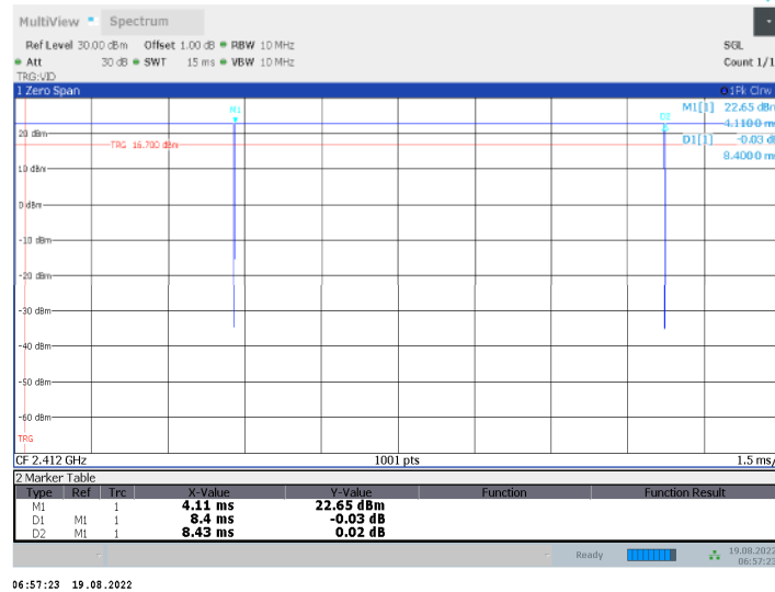
11G Ant2 2412
