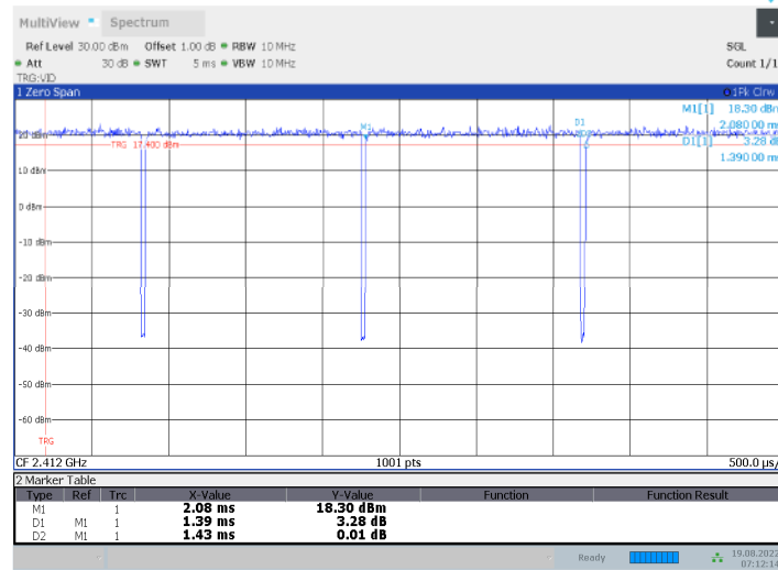
11G Ant2 2412
