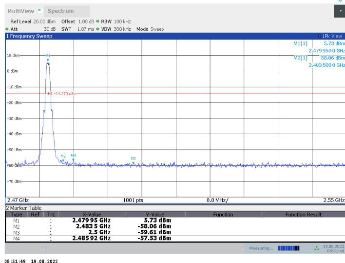
BLE_1M_Ant2_High_2480
