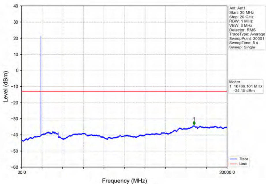
Band2_5MHz_64QAM_HCH_1907.5MHz_RB_1_24_NTNV
