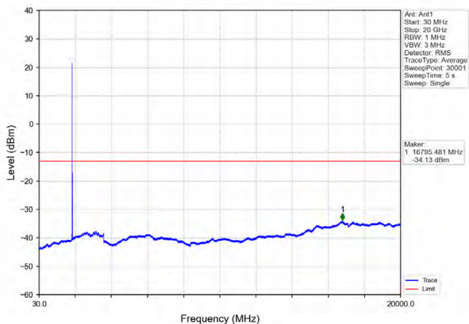
Band2_15MHz_64QAM_LCH_1857.5MHz_RB_1_0_NTNV
