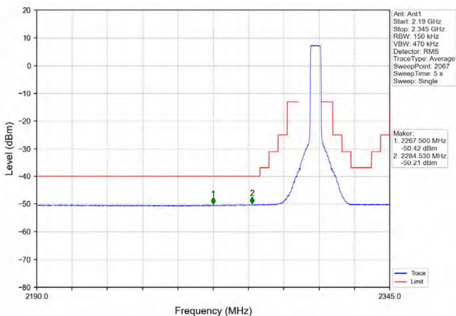
Band30_5MHz_64QAM_LCH_2307.5MHz_RB_1_0_NTNV
