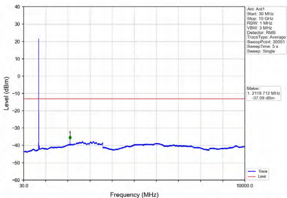
Band12_10MHz_16QAM_HCH_711MHz_RB_1_49_NTNV
