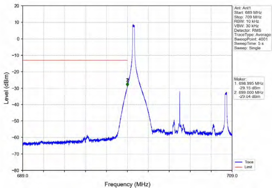
Band12_10MHz_64QAM_LCH_704MHz_RB_1_0_NTNV
