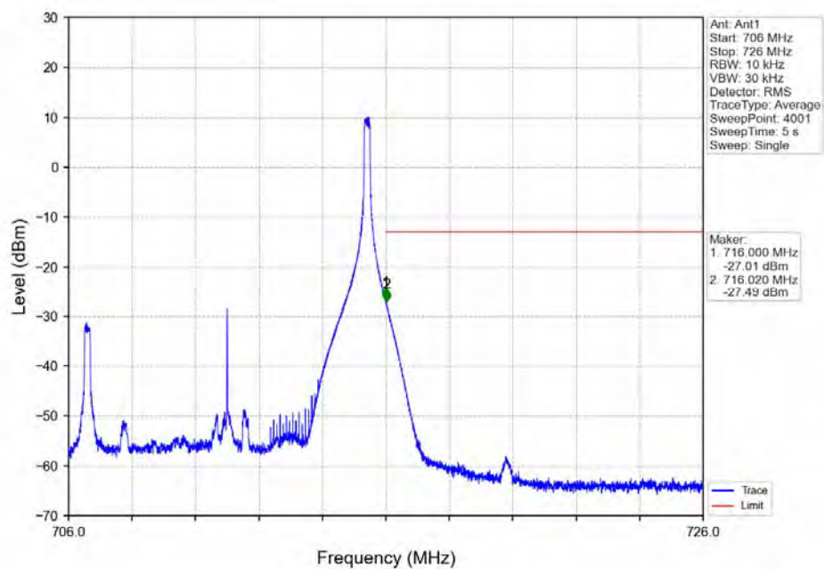
Band12_10MHz_16QAM_HCH_711MHz_RB_50_0_NTNV
