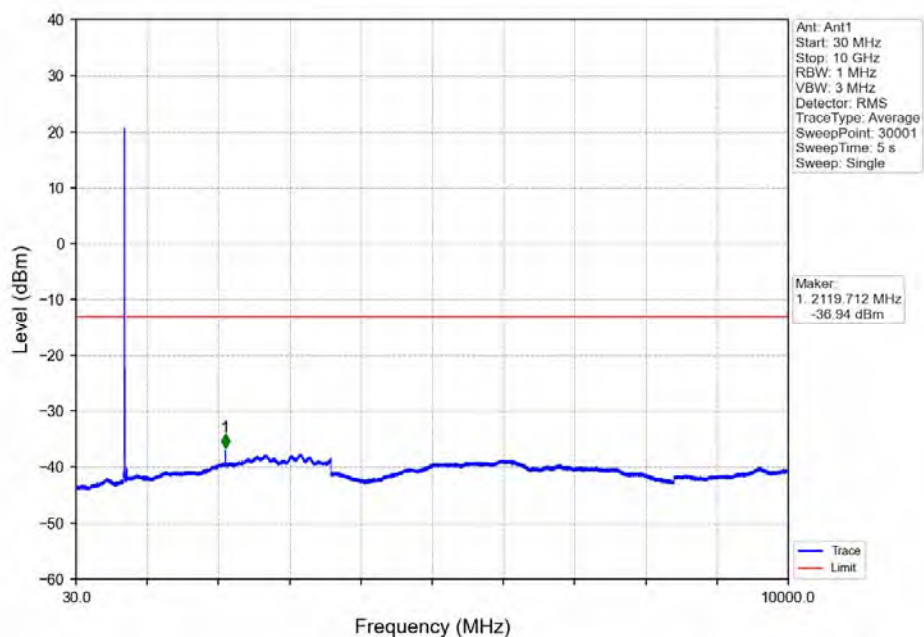
Band12_10MHz_64QAM_HCH_711MHz_RB_1_49_NTNV
