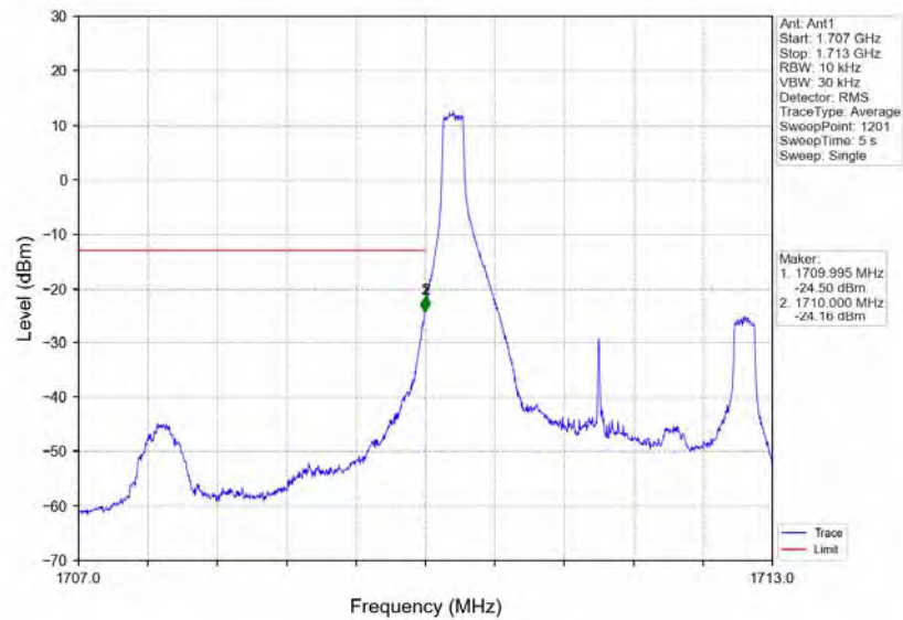
Band4_3MHz_QPSK_LCH_1711.5MHz_RB_1_0_NTNV
