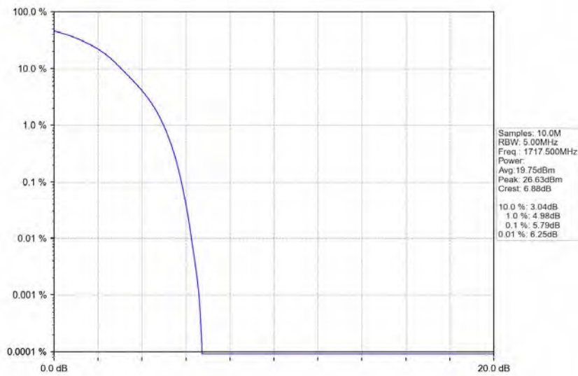
Band4_15MHz_QPSK_LCH_1717.5MHz_RB_75_0_NTNV
