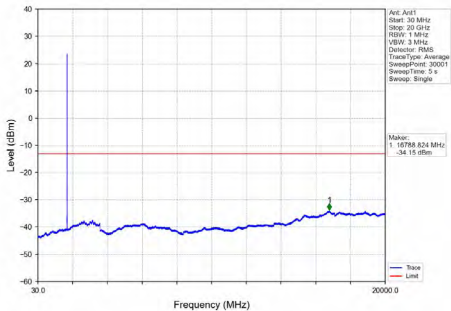
Band4_3MHz_QPSK_LCH_1711.5MHz_RB_1_0_NTNV
