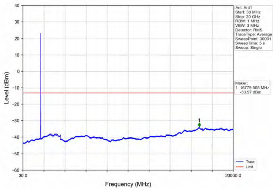
Band4_10MHz_QPSK_LCH_1715MHz_RB_1_0_NTNV
