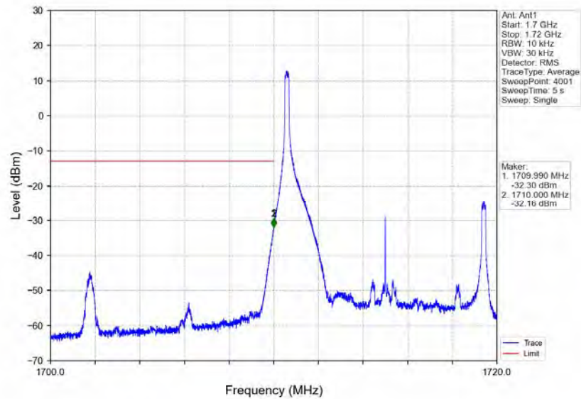
Band4_10MHz_QPSK_LCH_1715MHz_RB_1_0_NTNV
