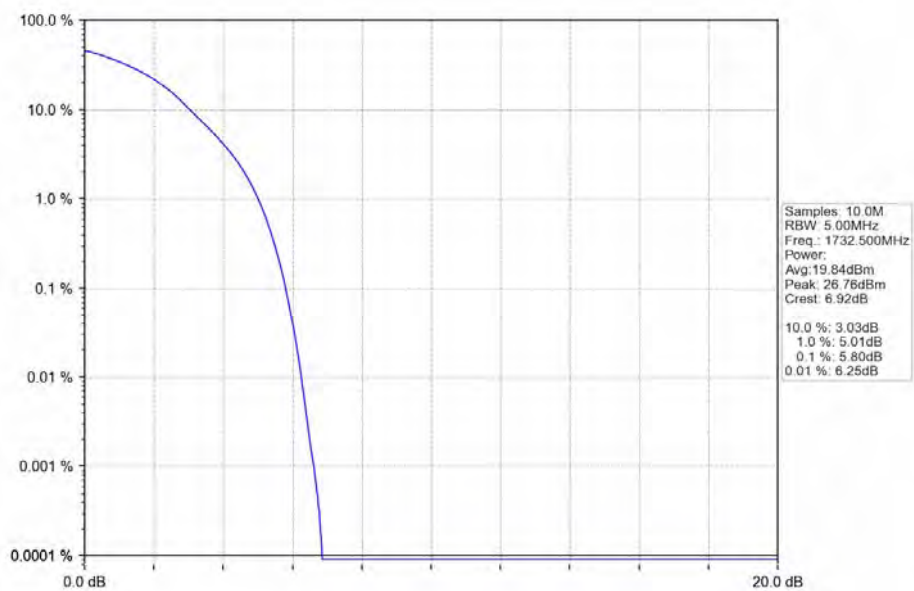
Band4_15MHz_QPSK_MCH_1732.5MHz_RB_75_0_NTNV
