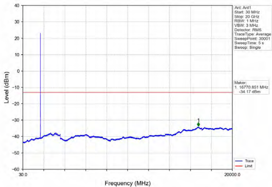
Band4_5MHz_QPSK_LCH_1712.5MHz_RB_1_0_NTNV
