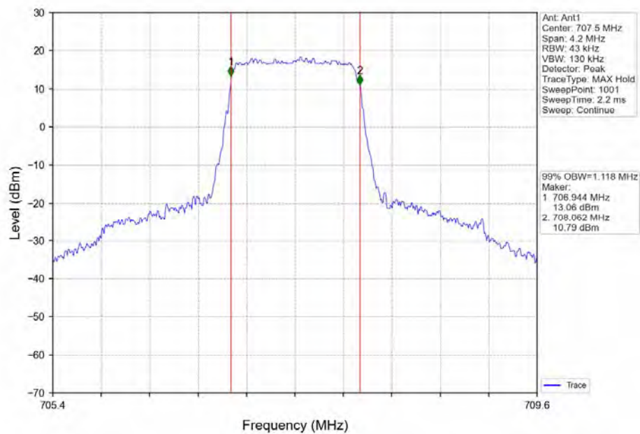
Band12_1.4MHz_QPSK_MCH_707.5MHz_RB_6_0_NTNV
