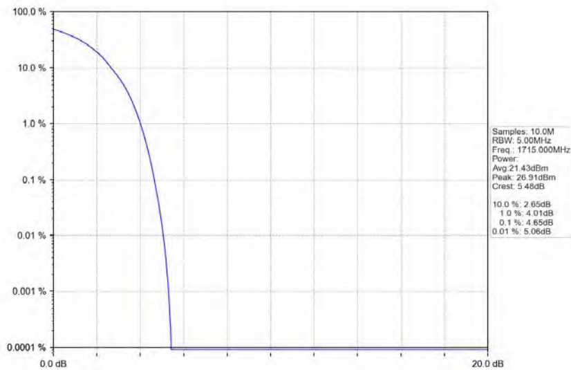
Band4_10MHz_QPSK_LCH_1715MHz_RB_50_0_NTNV
