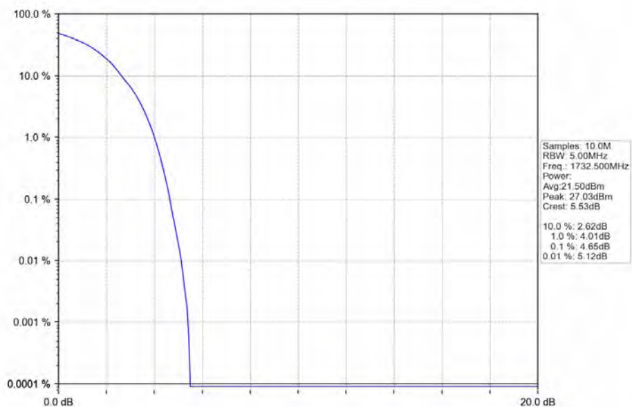
Band4_10MHz_QPSK_MCH_1732.5MHz_RB_50_0_NTNV
