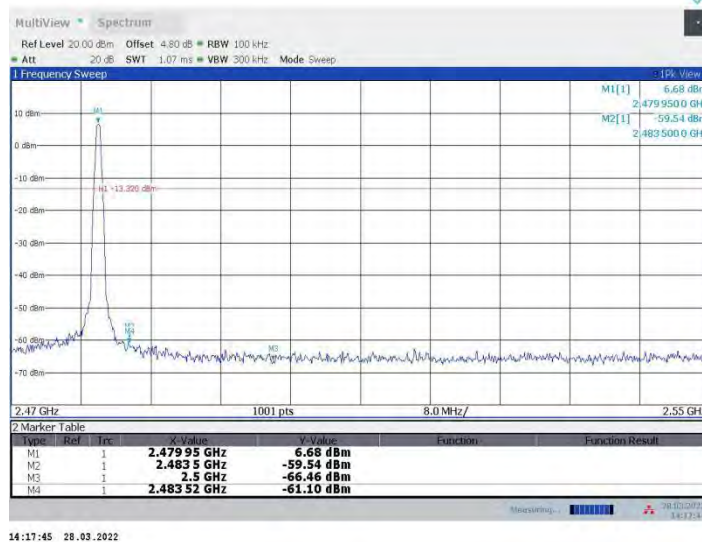
DH5_Ant 2_High_2480
