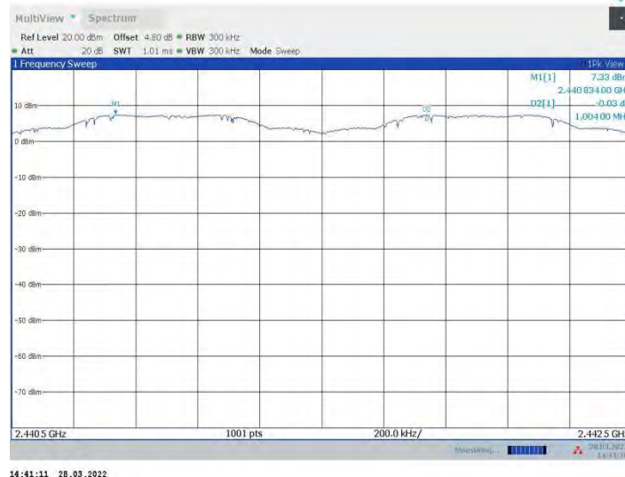
2DH5 Ant 2 Hop
