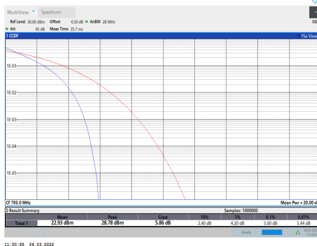
Band14-10MHz-16QAM-23330-50RB#0
