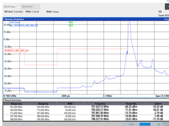
Band14-5MHz-QPSK-23305-25RB#0
