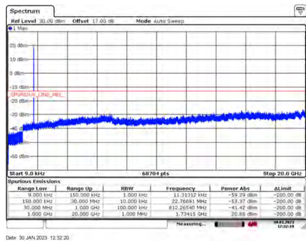
WCDMA Band IV CH-Middle 9kHz~20GHz
