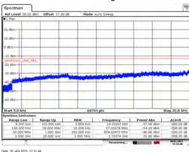
WCDMA Band IV CH-High 9kHz~20GHz
