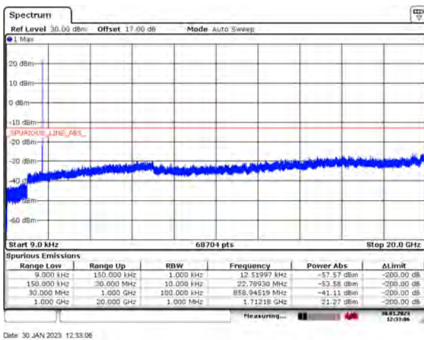
WCDMA Band IV CH-High 9kHz~20GHz
