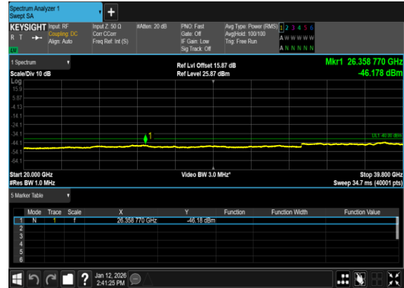
N77(100M)_DFT-s-OFDM_BPSK_Edge_1RB_Left_High_CH
