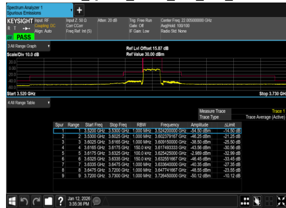
N77(15M)_DFT-s- OFDM_QPSK_Outer_Full_Mid_CH
