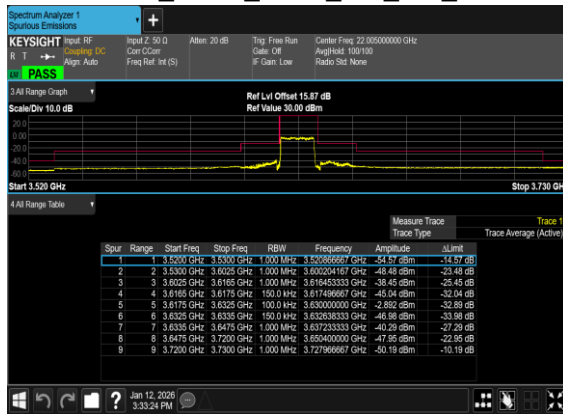
N77(15M)_DFT-s- OFDM_BPSK_Outer_Full_Mid_CH
