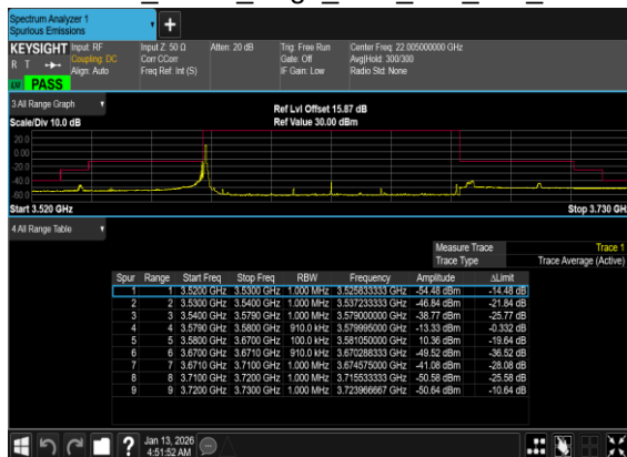
N77(90M)_DFT-s- OFDM_BPSK_Edge_1RB_Left_Mid_CH
