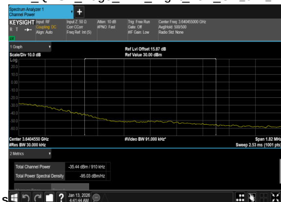
N77(90M)_DFT-s- OFDM_QPSK_Edge_1RB_Right_Low_CH_CHP_PAS
