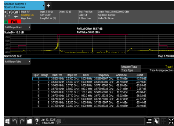
N77(90M)_DFT-s- OFDM_QPSK_Edge_1RB_Left_Mid_CH
