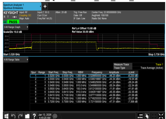
N77(90M)_DFT-s- OFDM_QPSK_Outer_Full_Low_CH
