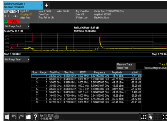
N77(90M)_DFT-s- OFDM_QPSK_Edge_1RB_Right_Low_CH
