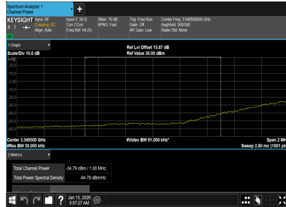
N77(100M)_DFT-s- OFDM_QPSK_Edge_1RB_Left_Low_CH_CHP_PASS
