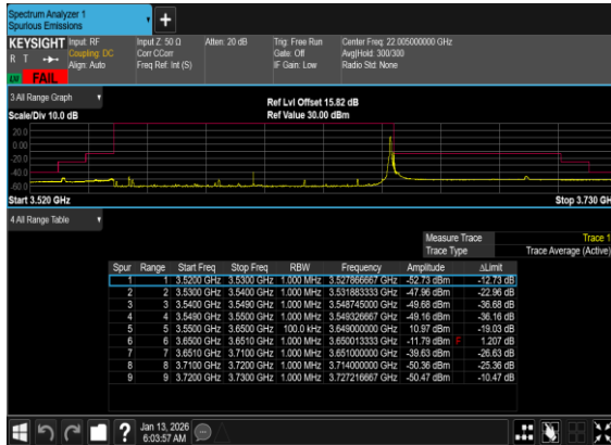
N77(100M)_DFT-s- OFDM_BPSK_Edge_1RB_Right_Low_CH
