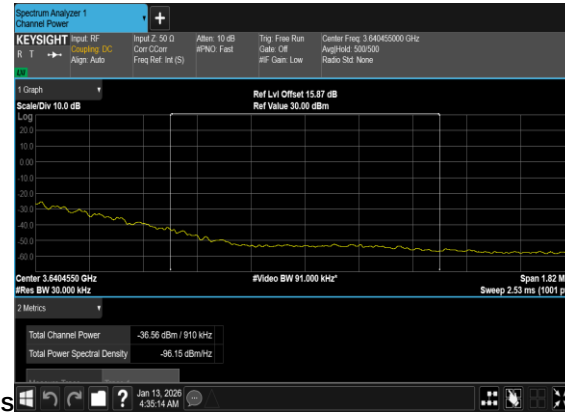
N77(90M)_DFT-s- OFDM_BPSK_Edge_1RB_Right_Low_CH_CHP_PAS
