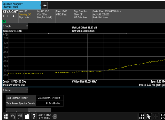
N77(90M)_DFT-s- OFDM_QPSK_Edge_1RB_Left_Mid_CH_CHP_PASS
