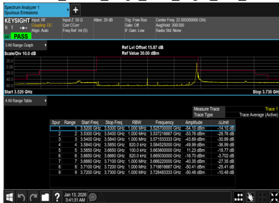
N77(80M)_DFT-s- OFDM_BPSK_Edge_1RB_Right_Mid_CH
