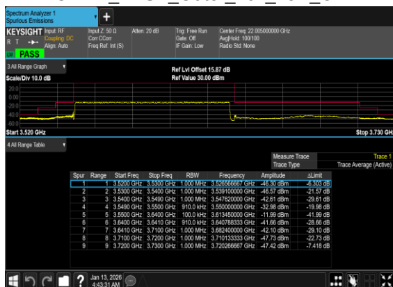
N77(90M)_DFT-s- OFDM_BPSK_Outer_Full_Low_CH
