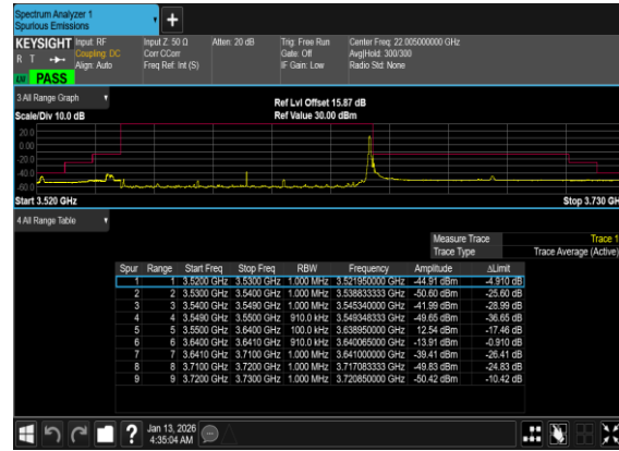
N77(90M)_DFT-s- OFDM_BPSK_Edge_1RB_Right_Low_CH
