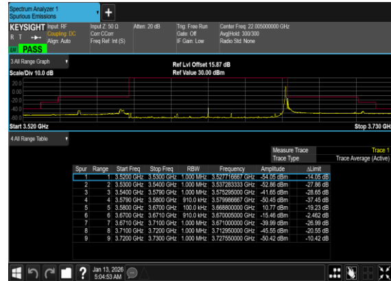
N77(90M)_DFT-s- OFDM_BPSK_Edge_1RB_Right_Mid_CH
