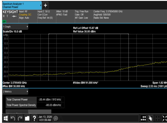
N77(90M)_DFT-s- OFDM_BPSK_Edge_1RB_Left_Mid_CH_CHP_PASS
