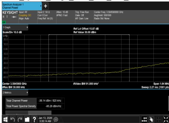
N77(80M)_DFT-s- OFDM_QPSK_Edge_1RB_Left_Mid_CH_CHP_PASS
