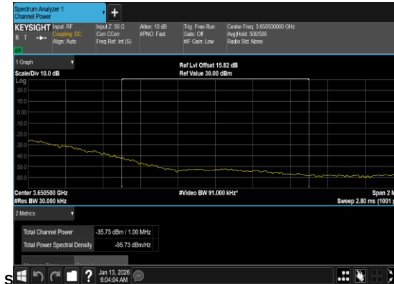
N77(100M)_DFT-s- OFDM_BPSK_Edge_1RB_Right_Low_CH_CHP_PAS
