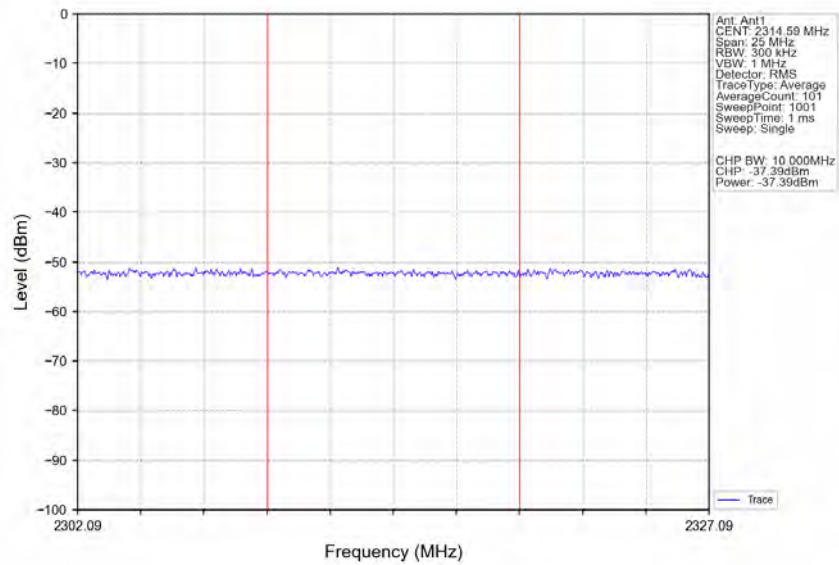
n30_15kHz_SISO_NTNV_10MHz_DFT-s-OFDM_PI/2_BPSK_2310MHz_Edge_1RB_Right_Ant1
