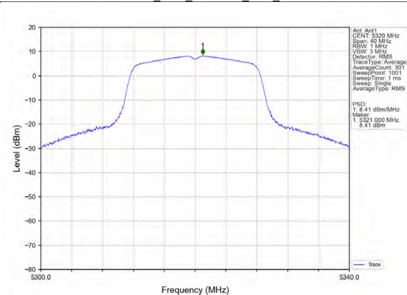
802.11a_HCH_5320MHz_Ant1_NTNV
