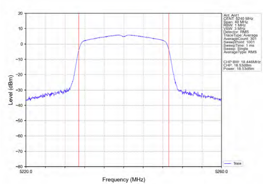
802.11ac(VHT20)_HCH_5240MHz_Ant1_NTNV
