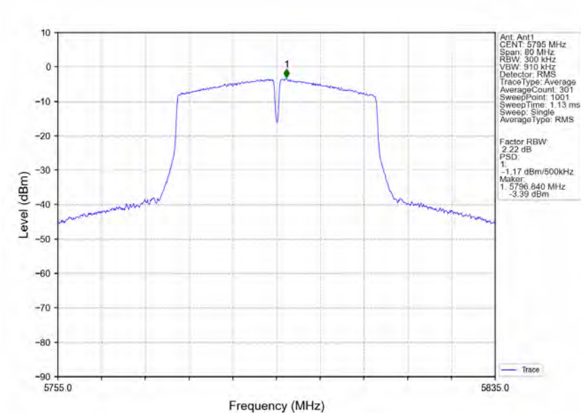
802.11ac(VHT40)_HCH_5795MHz_Ant1_NTNV
