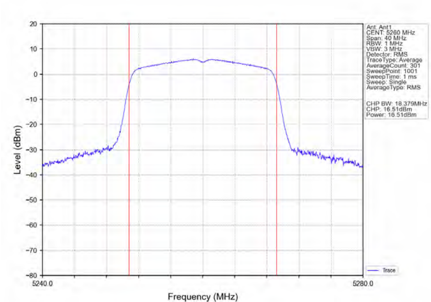
802.11ac(VHT20)_LCH_5260MHz_Ant1_NTNV
