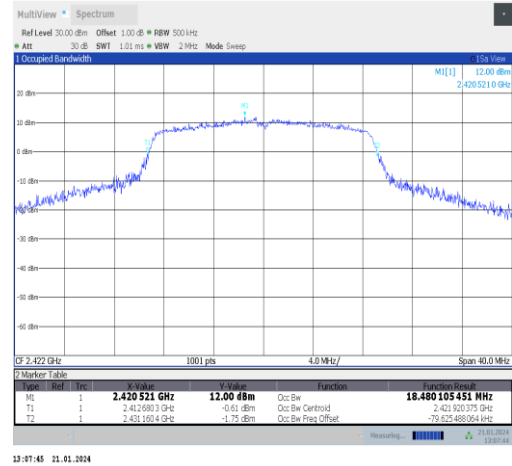
11n20SISO-Ant5-2422
