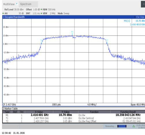
11n20SISO-Ant5-2417
