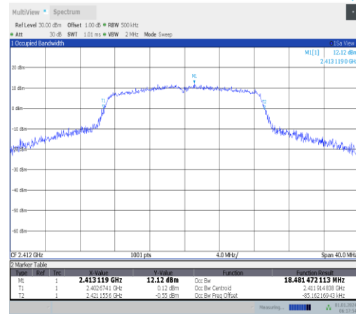
11n20SISO-Ant5-2412
