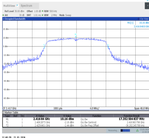
11g-Ant5-2417
