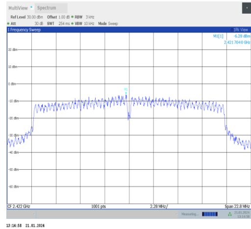
11n20SISO-Ant5-2422-PASS
