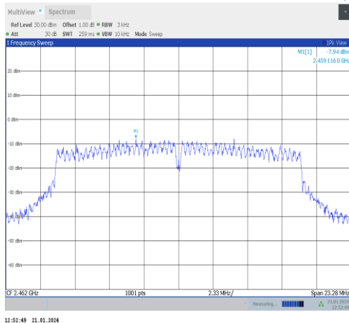
11g-Ant5-2462-PASS
