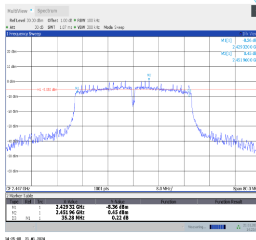
11n40SISO-Ant5-2447-PASS
