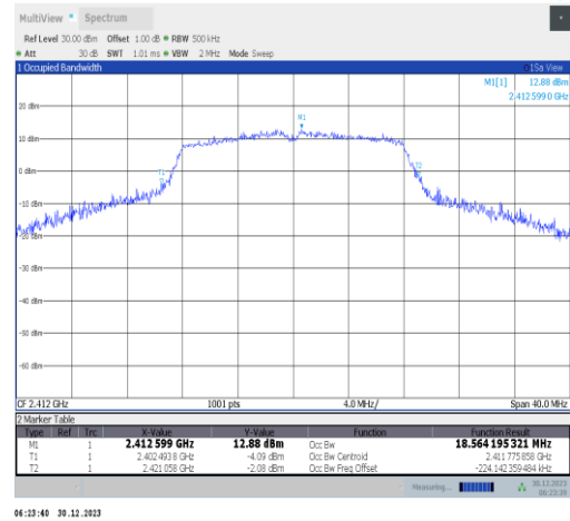
11g-Ant5-2412
