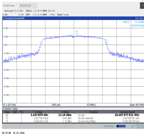
11n20SISO-Ant5-2437
