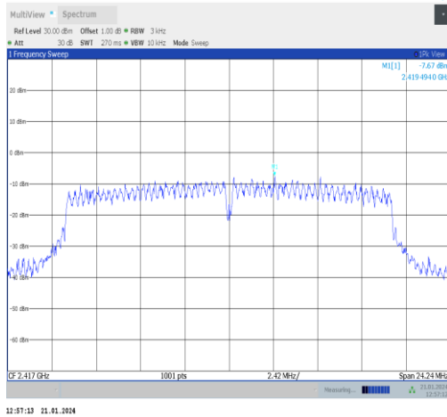
11n20SISO-Ant5-2417-PASS
