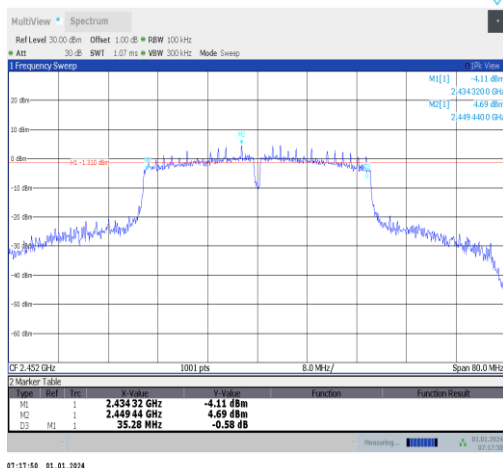
11n40SISO-Ant5-2452-PASS
