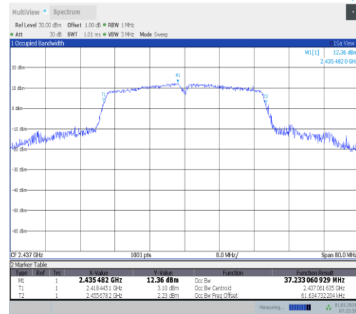
11n40SISO-Ant5-2437
