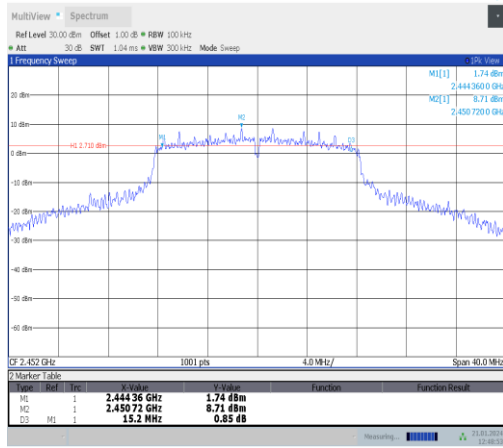
11g-Ant5-2452-PASS
