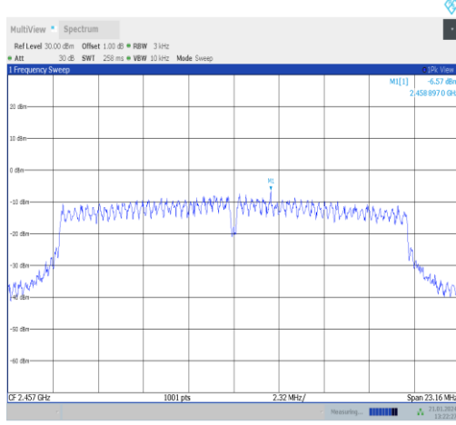
11n20SISO-Ant5-2457-PASS
