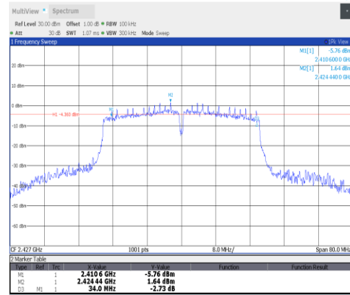
11n40SISO-Ant5-2427-PASS
