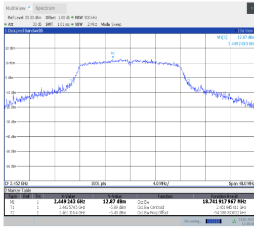
11g-Ant5-2452
