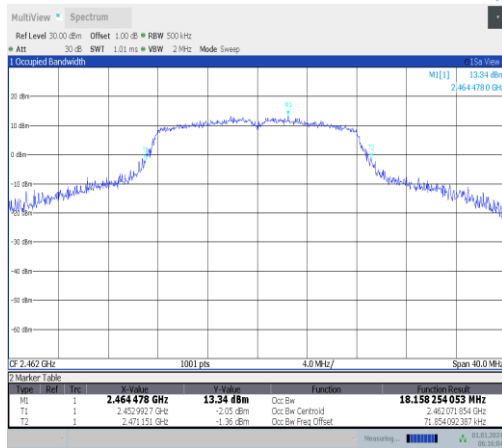
11g-Ant5-2462
