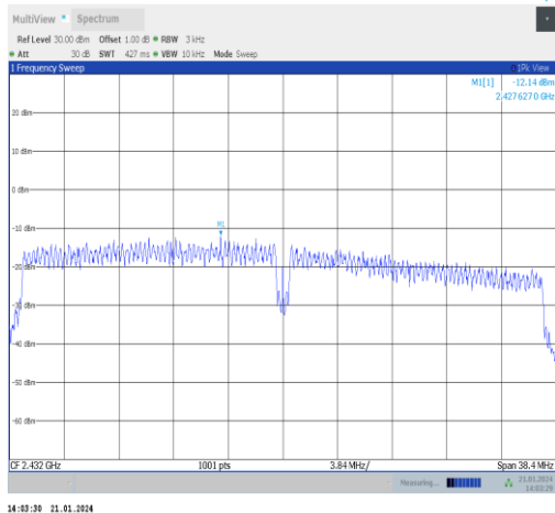
11n40SISO-Ant5-2432-PASS
