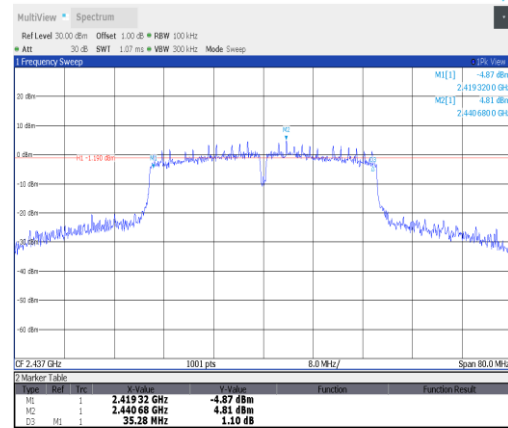
11n40SISO-Ant5-2437-PASS
