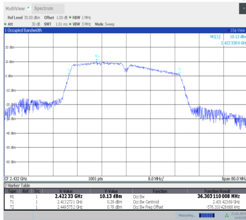
11n40SISO-Ant5-2432
