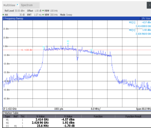
11n40SISO-Ant5-2432-PASS
