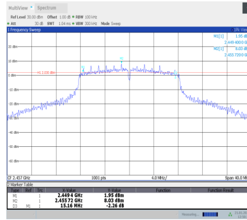
11g-Ant5-2457-PASS
