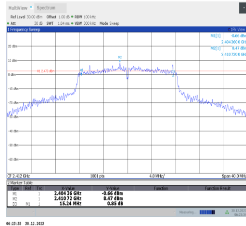
11g-Ant5-2412-PASS
