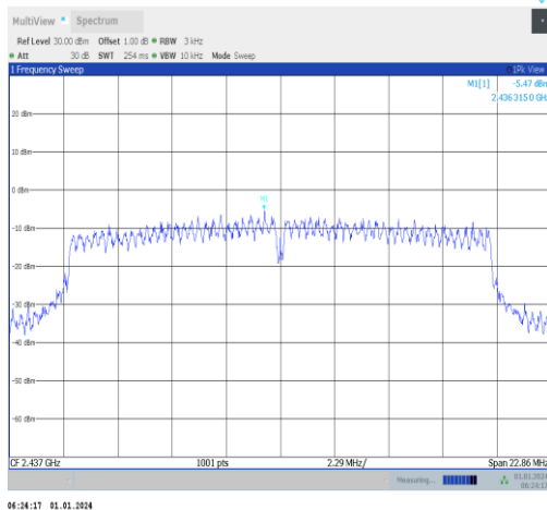
11n20SISO-Ant5-2437-PASS
