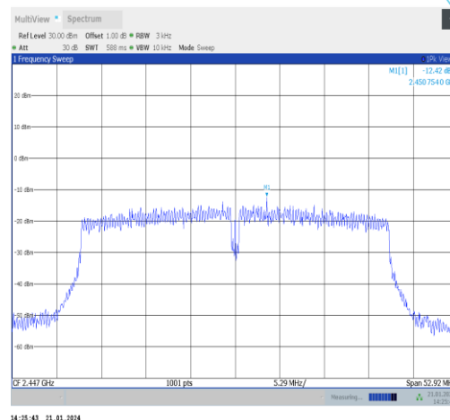
11n40SISO-Ant5-2447-PASS
