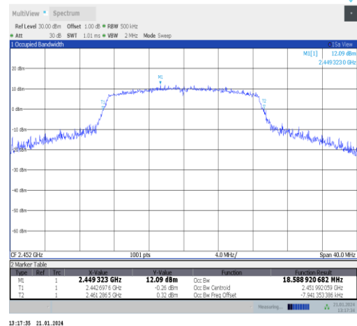
11n20SISO-Ant5-2452
