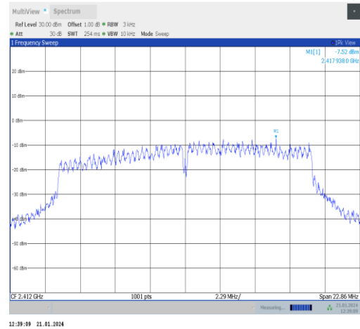
11g-Ant5-2412-PASS
