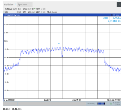
11g-Ant5-2422-PASS
