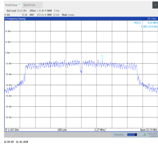
11g-Ant5-2457-PASS
