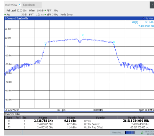
11n40SISO-Ant5-2427
