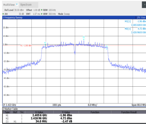
11n40SISO-Ant5-2422-PASS
