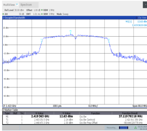
11n40SISO-Ant5-2422
