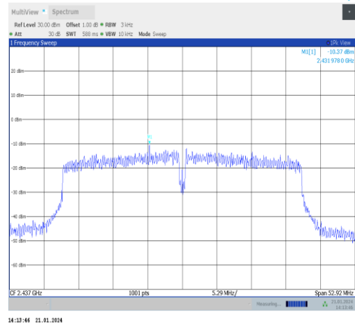
11n40SISO-Ant5-2437-PASS
