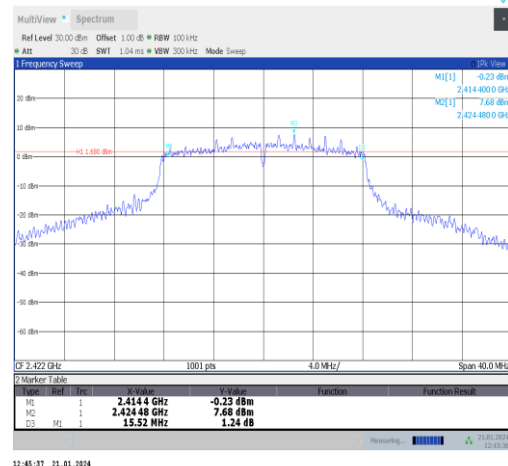
11g-Ant5-2422-PASS
