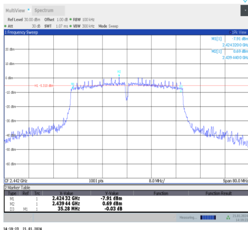
11n40SISO-Ant5-2442-PASS
