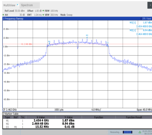
11g-Ant5-2462-PASS
