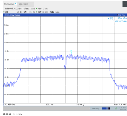
11n40SISO-Ant5-2427-PASS
