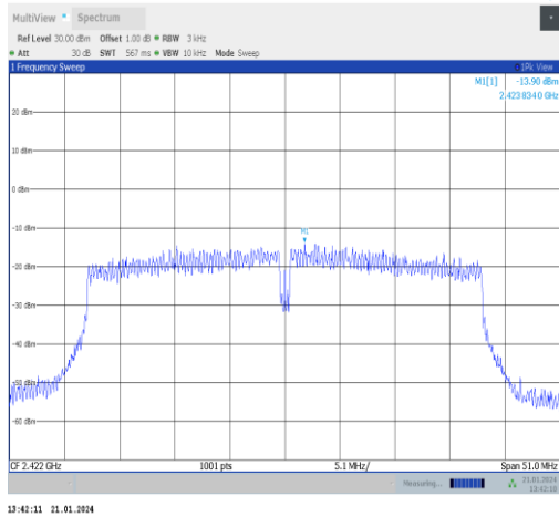
11n40SISO-Ant5-2422-PASS
