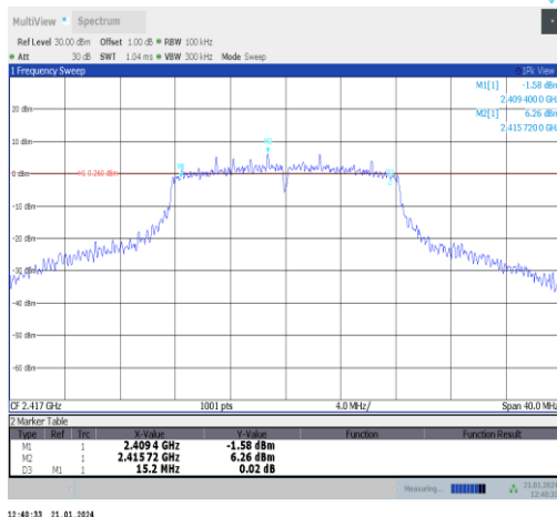
11g-Ant5-2417-PASS
