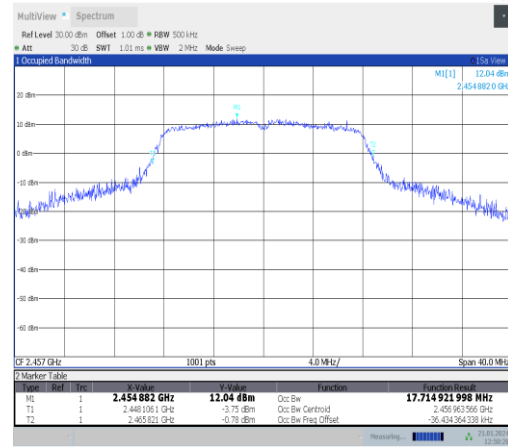
11g-Ant5-2457
