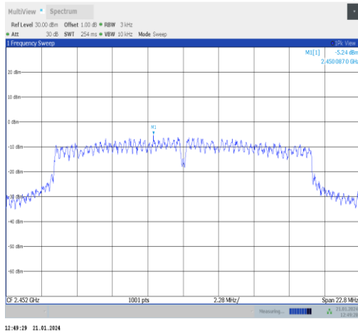
11g-Ant5-2452-PASS
