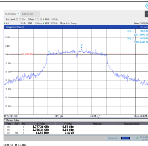
11a-Ant5-5785-PASS
