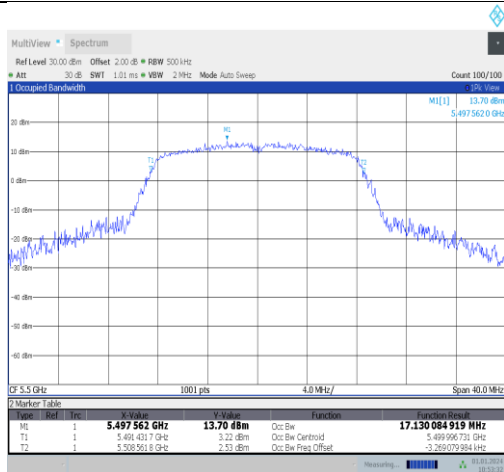
11a-Ant5-5500
