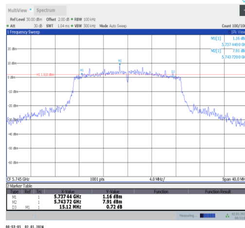
11n20SISO-Ant5-5745-PASS
