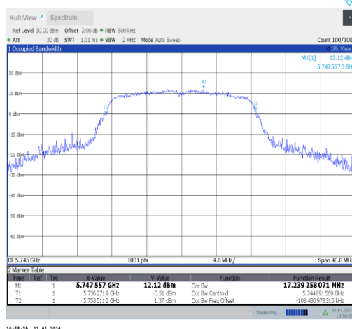
11a-Ant5-5745
