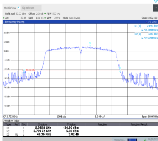
11n40SISO-Ant5-5795
