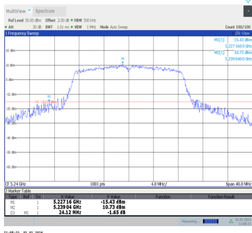
11n20SISO-Ant5-5240
