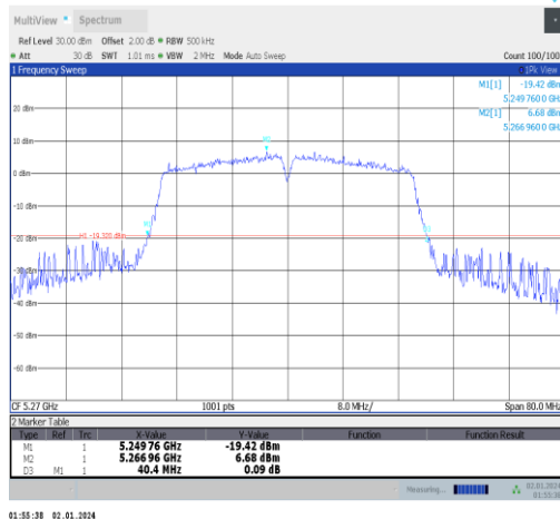
11n40SISO-Ant5-5270
