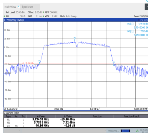
11n40SISO-Ant5-5755
