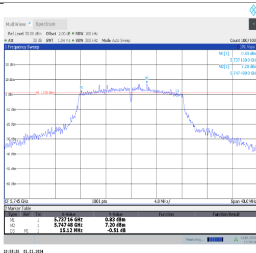
11a-Ant5-5745-PASS
