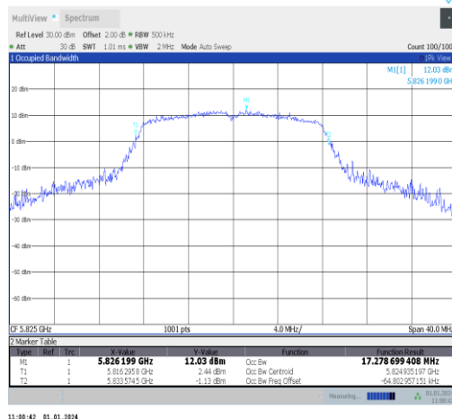
11a-Ant5-5825
