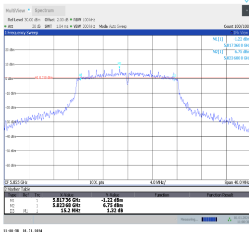
11a-Ant5-5825-PASS
