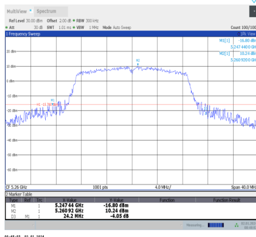
11n20SISO-Ant5-5260
