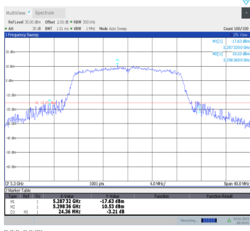
11n20SISO-Ant5-5300
