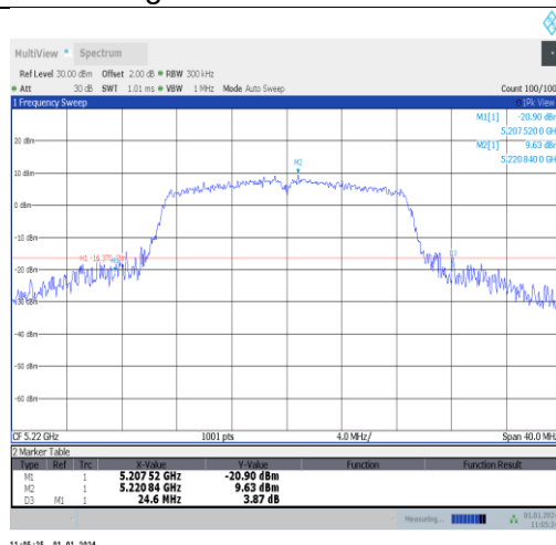
11n20SISO-Ant5-5220
