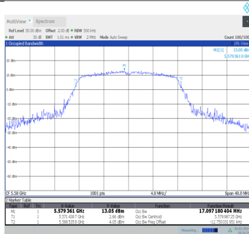
11a-Ant5-5580
