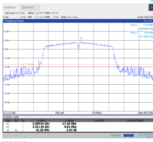
11n40SISO-Ant5-5510
