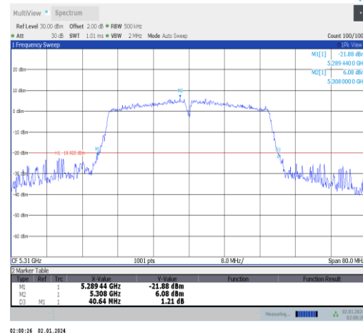
11n40SISO-Ant5-5310
