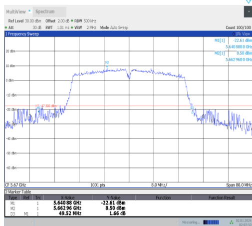
11n40SISO-Ant5-5670
