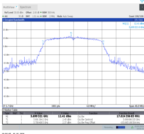
11a-Ant5-5700
