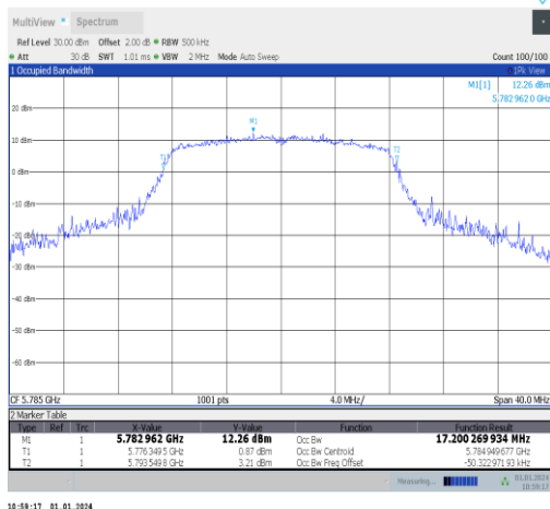
11a-Ant5-5785
