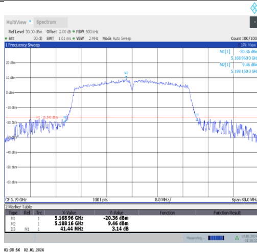
11n40SISO-Ant5-5190
