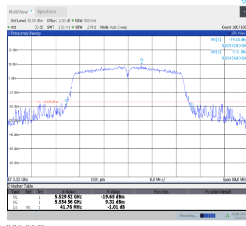
11n40SISO-Ant5-5550
