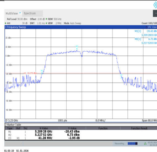
11n40SISO-Ant5-5230
