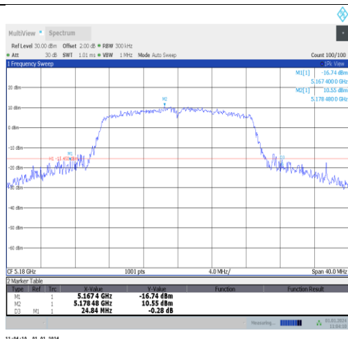
11n20SISO-Ant5-5180
