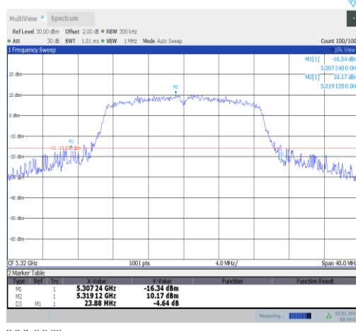
11n20SISO-Ant5-5320
