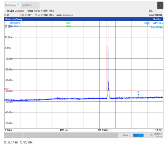
1-N30-30-10-M-1-DFT-PI2BPSK-Inner_1RB_Left-1@ 1-1000-3000-Ant3-2689.00--44.51--40-PASS
