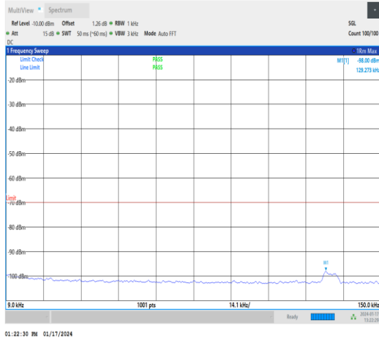
1-N30-30-10-H-1-DFT-PI2BPSK-Inner_1RB_Left-1 @1-0.009-0.15-Ant3-0.13--98.00--70-PASS
