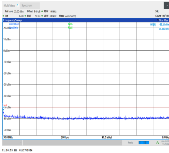
1-N30-30-10-M-1-DFT-PI2BPSK-Inner_1RB_Left-1 @ 1-30-1000-Ant3-35.34--53.20--50-PASS
