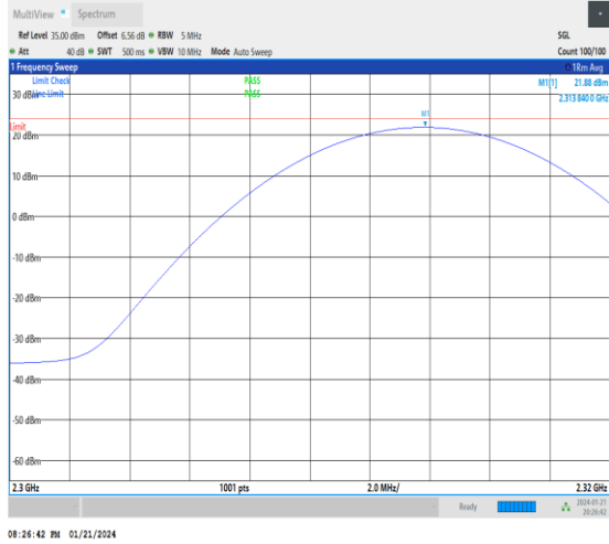
1-N30-30-10-M-2-DFT-PI2BPSK-Inner_1RB_Right-1 @22-2300-2320-Ant3-2313.84-21.88-23.98-PASS
