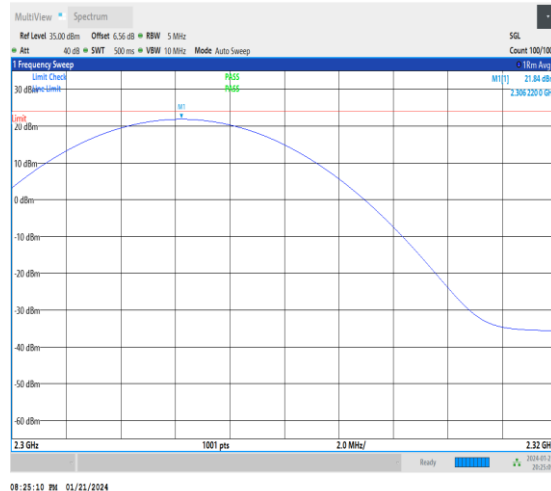
1-N30-30-10-M-1-DFT-PI2BPSK-Inner_1RB_Left-1 @1-2300-2320-Ant3-2306.22-21.84-23.98-PASS
