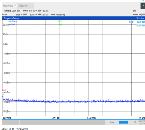
1-N30-30-10-H-1-DFT-PI2BPSK-Inner_1RB_Left-1 @1-30-1000-Ant3-35.34--53.88--50-PASS
