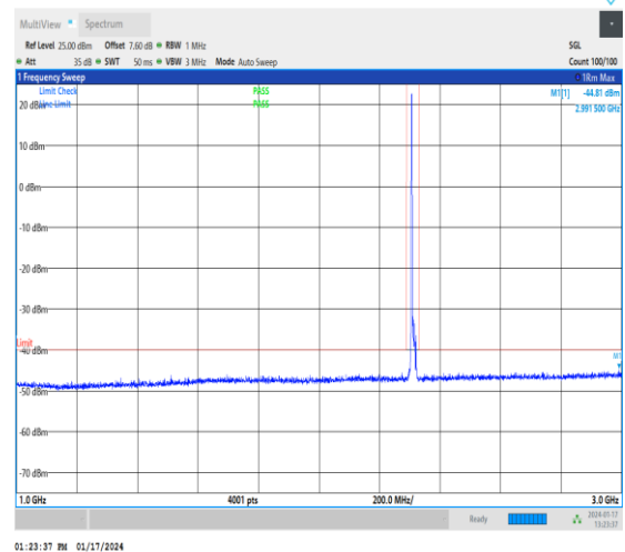
1-N30-30-10-H-1-DFT-PI2BPSK-Inner_1RB_Left-1@ 1-1000-3000-Ant3-2991.50--44.81--40-PASS
