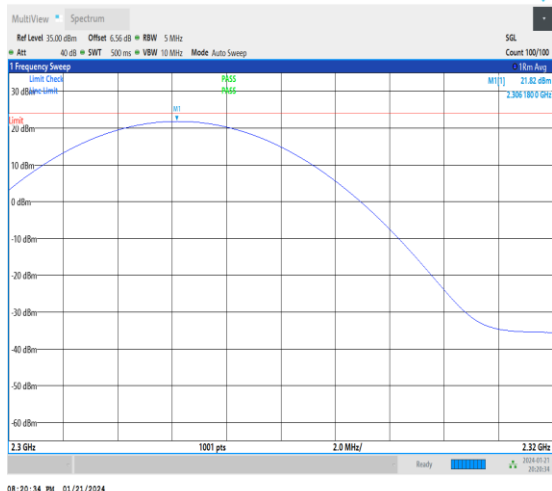
1-N30-30-10-L-1-DFT-PI2BPSK-Inner_1RB_Left-1@ 1-2300-2320-Ant3-2306.18-21.82-23.98-PASS
