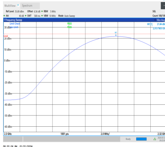
1-N30-30-10-L-2-DFT-PI2BPSK-Inner_1RB_Right-1 @22-2300-2320-Ant3-2313.76-21.84-23.98-PASS
