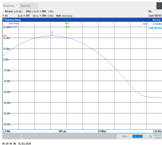
1-N30-30-10-H-1-DFT-PI2BPSK-Inner_1RB_Left-1@ 1-2300-2320-Ant3-2306.20-21.86-23.98-PASS
