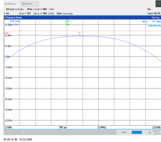
1-N30-30-10-M-3-DFT-PI2BPSK-Outer_Full-24@0-2 300-2320-Ant3-2309.62-19.17-23.98-PASS
