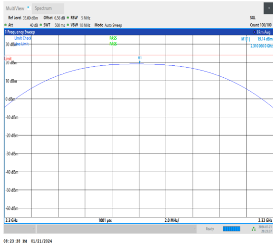
1-N30-30-10-L-3-DFT-PI2BPSK-Outer_Full-24@0-23 00-2320-Ant3-2310.06-19.14-23.98-PASS
