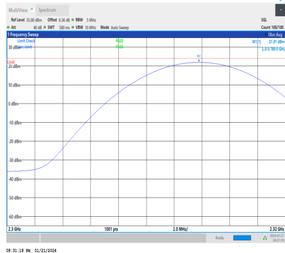
1-N30-30-10-H-2-DFT-PI2BPSK-Inner_1RB_Right-1 @22-2300-2320-Ant3-2313.78-21.91-23.98-PASS
