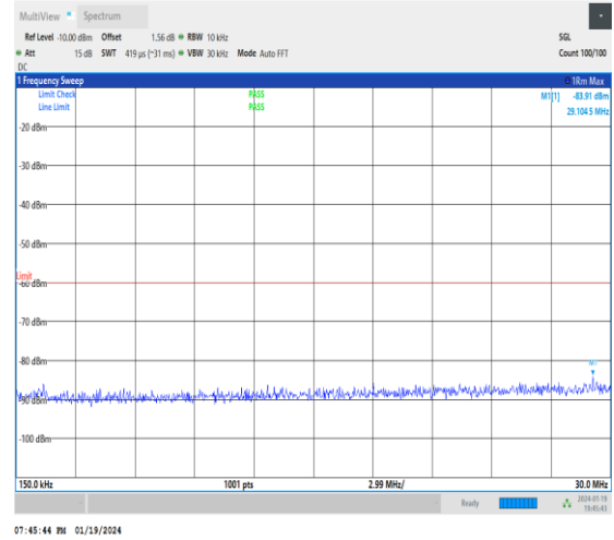
1-N30-30-10-H-1-DFT-PI2BPSK-Inner_1RB_Left-1@ 1-0.15-30-Ant3-29.10--83.91--60-PASS
