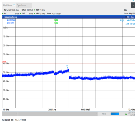
1-N30-30-10-M-1-DFT-PI2BPSK-Inner_1RB_Left-1 @ 1-3000-12000-Ant3-7389.75--46.07--40-PASS
