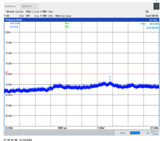
1-N30-30-10-M-1-DFT-PI2BPSK-Inner_1RB_Left-1@ 1-12000-27000-Ant3-22247.00--46.43--40-PASS
