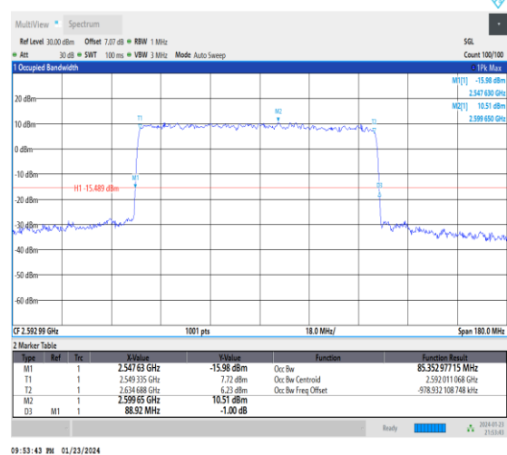
1-N41-30-90-M-1-DFT-QPSK-Outer_Full-240@0-Ant 3-85.353-88.920-≤90-PASS
