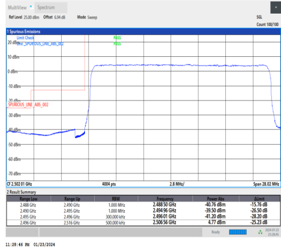
1-N41-30-20-L-3-DFT-PI2BPSK-Outer_Full-50@0-Ant3-1--PASS-see graph
