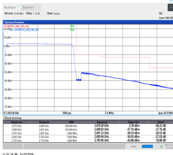
1-N41-30-15-H-6-CP-QPSK-Outer_Full-38@0-Ant3-1--PASS-see graph
