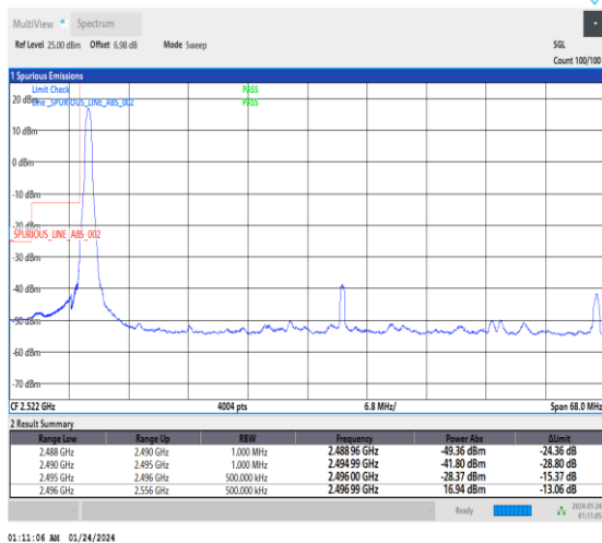
1-N41-30-60-L-4-CP-QPSK-Edge_1RB_Left-1@0-Ant3-1--PASS-see graph
