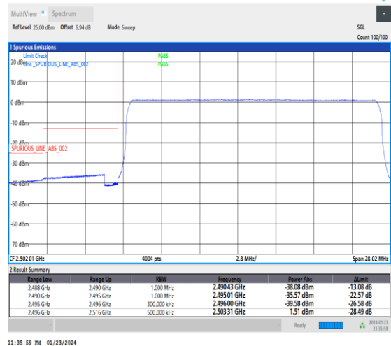
1-N41-30-20-L-6-CP-QPSK-Outer_Full-51@0-Ant3-1--PASS-see graph
