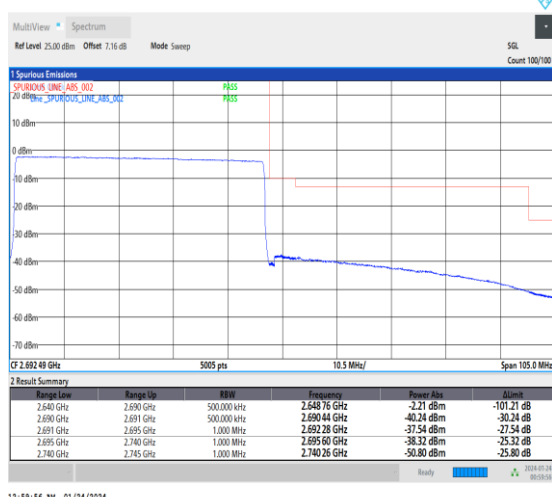
1-N41-30-50-H-6-CP-QPSK-Outer_Full-133@0-Ant3-1--PASS-see graph
