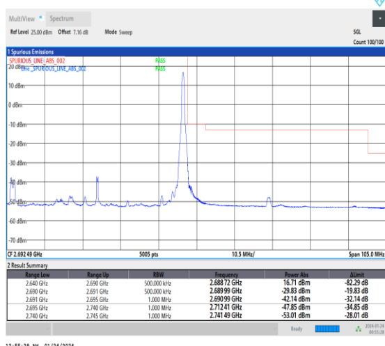
1-N41-30-50-H-5-CP-QPSK-Edge_1RB_Right-1@132-Ant3-1--PASS-see graph
