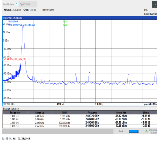
1-N41-30-60-L-1-DFT-PI2BPSK-Edge_1RB_Left-1@0-Ant3-1--PASS-see graph
