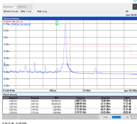
1-N41-30-50-H-2-DFT-PI2BPSK-Edge_1RB_Right-1@132-Ant3-1--PASS-see graph
