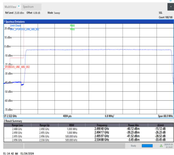
1-N41-30-60-L-6-CP-QPSK-Outer_Full-162@0-Ant3-1--PASS-see graph
