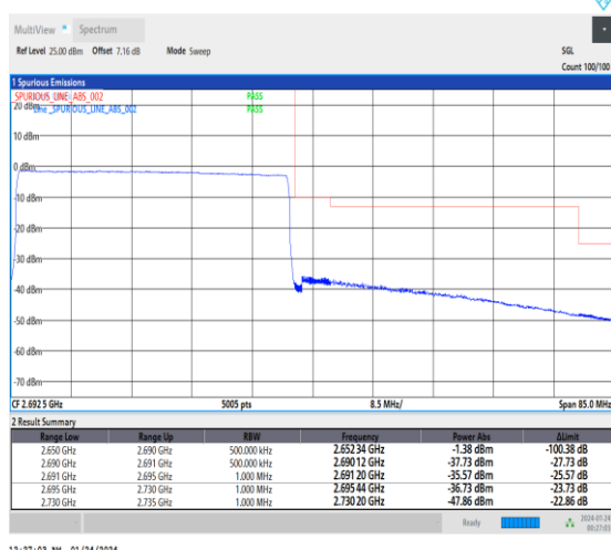
1-N41-30-40-H-6-CP-QPSK-Outer_Full-106@0-Ant3-1--PASS-see graph
