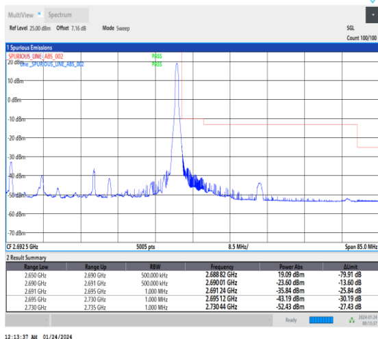
1-N41-30-40-H-2-DFT-PI2BPSK-Edge_1RB_Right-1@105-Ant3-1--PASS-see graph
