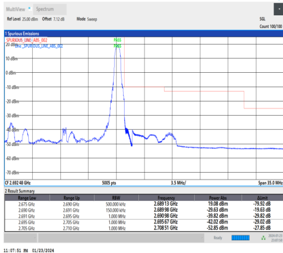
1-N41-30-15-H-2-DFT-PI2BPSK-Edge_1RB_Right-1@37-Ant3-1--PASS-see graph
