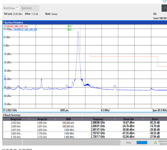
1-N41-30-40-H-5-CP-QPSK-Edge_1RB_Right-1@105-Ant3-1--PASS-see graph
