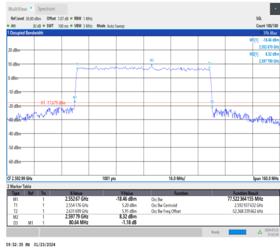
1-N41-30-80-M-8-CP-64QAM-Outer_Full-217@0-Ant 3-77.522-80.640-≤80-PASS
