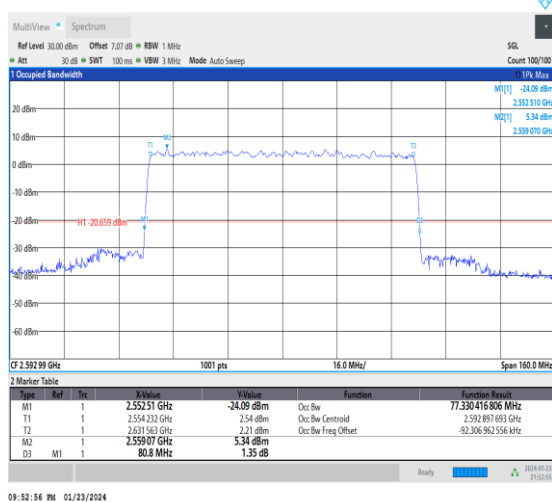
1-N41-30-80-M-9-CP-256QAM-Outer_Full-217@0-A nt3-77.33-80.800-≤80-PASS
