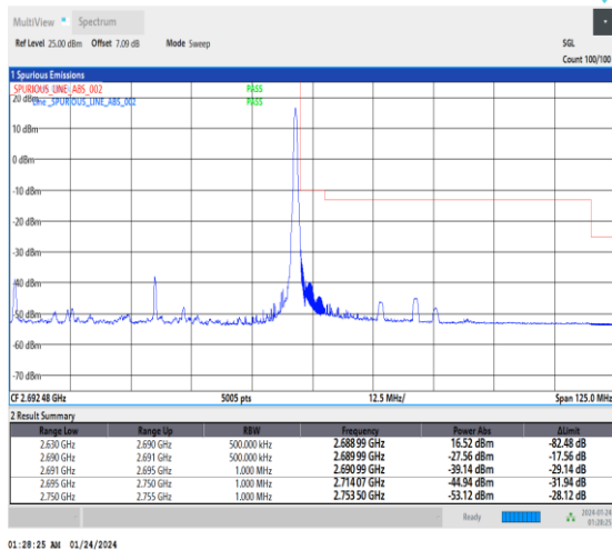
1-N41-30-60-H-5-CP-QPSK-Edge_1RB_Right-1@161-Ant3-1--PASS-see graph
