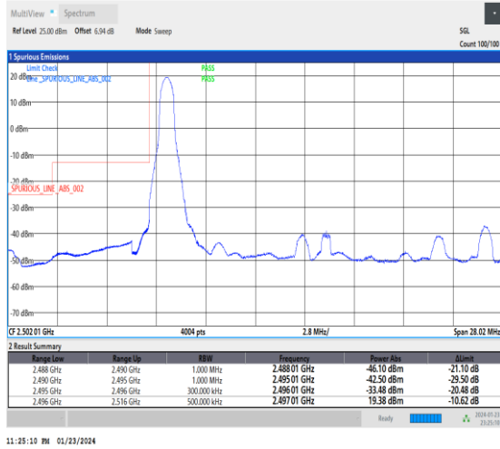
1-N41-30-20-L-1-DFT-PI2BPSK-Edge_1RB_Left-1@0-Ant3-1--PASS-see graph
