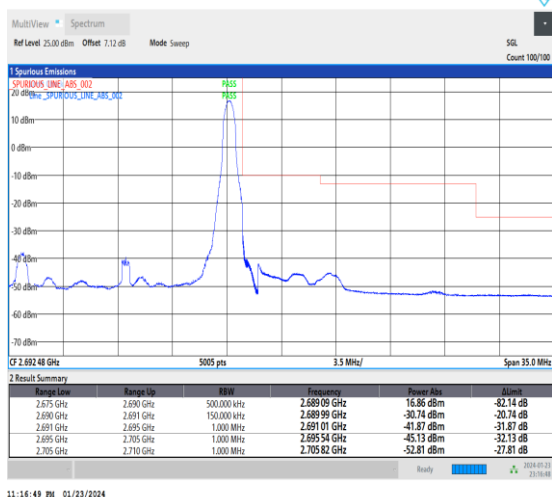
1-N41-30-15-H-5-CP-QPSK-Edge_1RB_Right-1@37-Ant3-1--PASS-see graph
