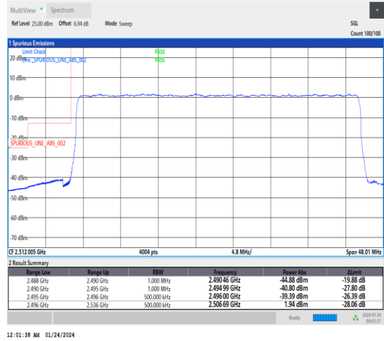
1-N41-30-40-L-3-DFT-PI2BPSK-Outer_Full-100@0-Ant3-1--PASS-see graph
