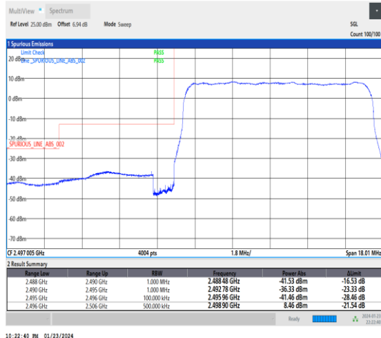
1-N41-30-10-L-3-DFT-PI2BPSK-Outer_Full-24@0-Ant3-1--PASS-see graph
