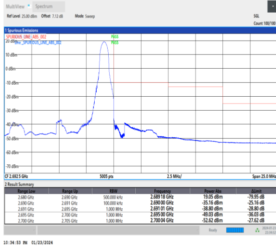
1-N41-30-10-H-2-DFT-PI2BPSK-Edge_1RB_Right-1@23-Ant3-1--PASS-see graph
