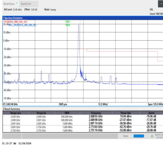
1-N41-30-60-H-2-DFT-PI2BPSK-Edge_1RB_Right-1@161-Ant3-1--PASS-see graph
