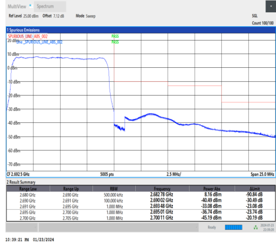
1-N41-30-10-H-3-DFT-PI2BPSK-Outer_Full-24@0-Ant3-1--PASS-see graph
