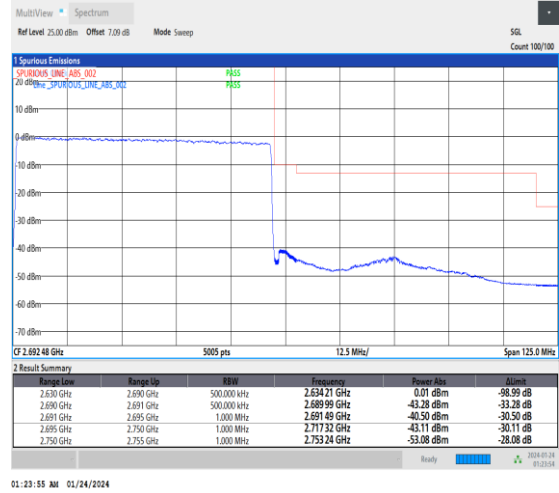
1-N41-30-60-H-3-DFT-PI2BPSK-Outer_Full-162@0-Ant3-1--PASS-see graph
