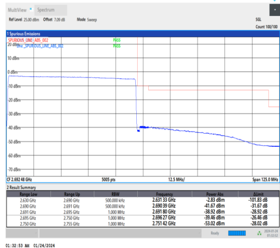
1-N41-30-60-H-6-CP-QPSK-Outer_Full-162@0-Ant3-1--PASS-see graph
