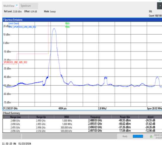
1-N41-30-20-L-4-CP-QPSK-Edge_1RB_Left-1@0-Ant3-1--PASS-see graph
