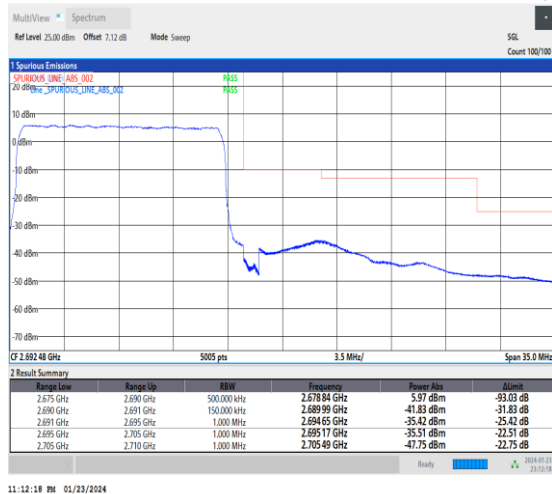
1-N41-30-15-H-3-DFT-PI2BPSK-Outer_Full-36@0-Ant3-1--PASS-see graph
