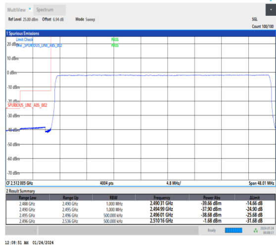
1-N41-30-40-L-6-CP-QPSK-Outer_Full-106@0-Ant3-1--PASS-see graph
