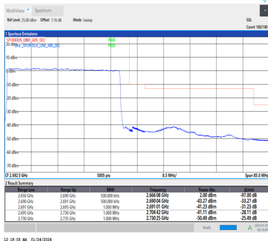
1-N41-30-40-H-3-DFT-PI2BPSK-Outer_Full-100@0-Ant3-1--PASS-see graph
