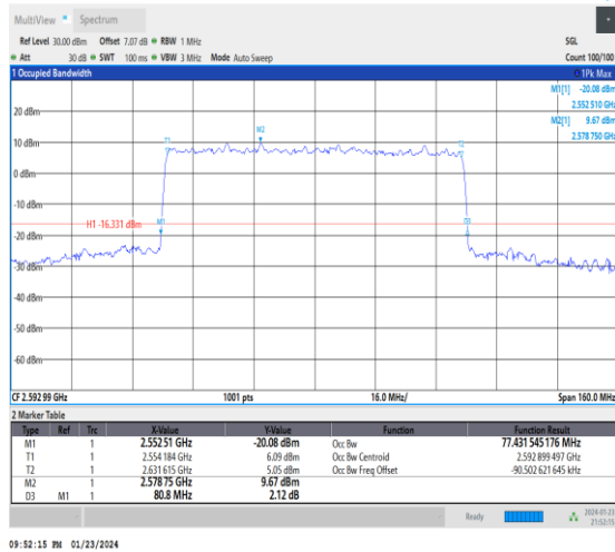
1-N41-30-80-M-7-CP-16QAM-Outer_Full-217@0-An t3-77.432-80.800≤80-PASS
