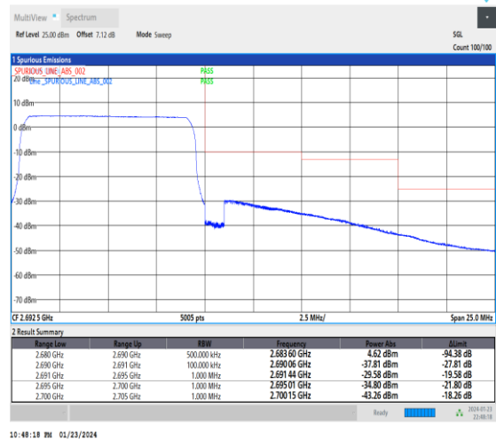
1-N41-30-10-H-6-CP-QPSK-Outer_Full-24@0-Ant3-1--PASS-see graph
