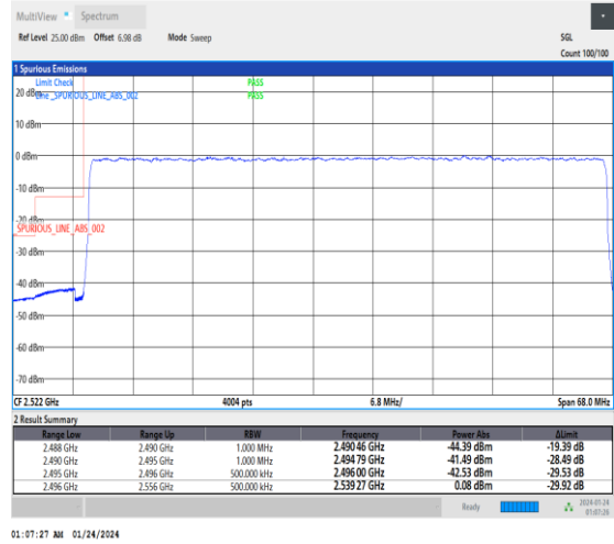
1-N41-30-60-L-3-DFT-PI2BPSK-Outer_Full-162@0-Ant3-1--PASS-see graph
