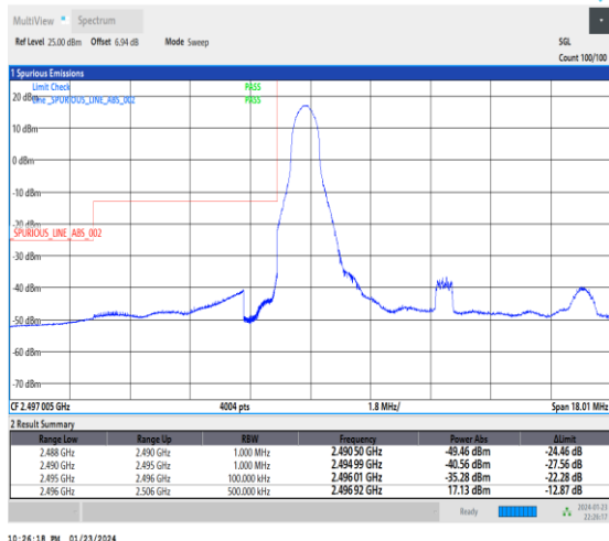
1-N41-30-10-L-4-CP-QPSK-Edge_1RB_Left-1@0-Ant3-1--PASS-see graph
