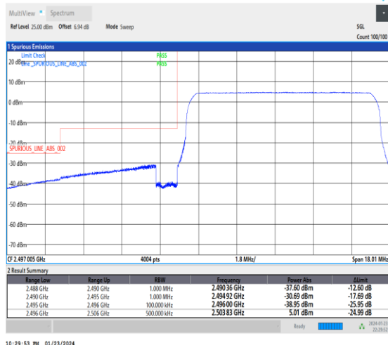
1-N41-30-10-L-6-CP-QPSK-Outer_Full-24@0-Ant3-1--PASS-see graph
