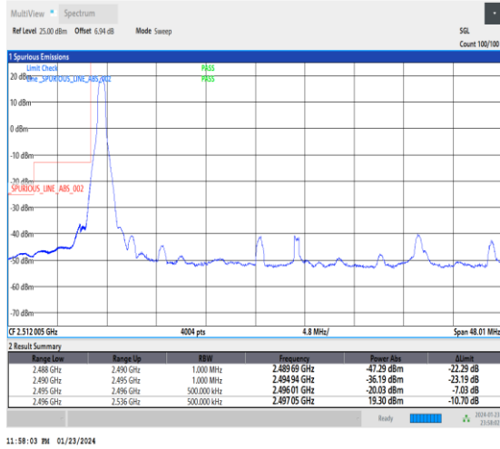
1-N41-30-40-L-1-DFT-PI2BPSK-Edge_1RB_Left-1@0-Ant3-1--PASS-see graph
