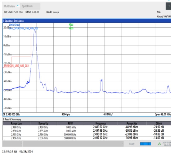
1-N41-30-40-L-4-CP-QPSK-Edge_1RB_Left-1@0-Ant3-1--PASS-see graph
