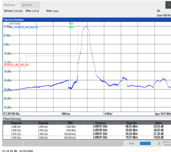
1-N41-30-10-L-1-DFT-PI2BPSK-Edge_1RB_Left-1@0-Ant3-1--PASS-see graph
