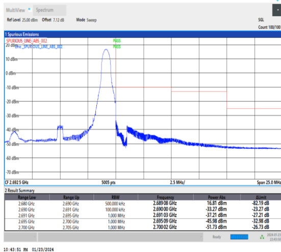
1-N41-30-10-H-5-CP-QPSK-Edge_1RB_Right-1@23-Ant3-1--PASS-see graph
