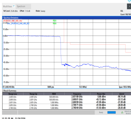
1-N41-30-50-H-3-DFT-PI2BPSK-Outer_Full-128@0-Ant3-1--PASS-see graph
