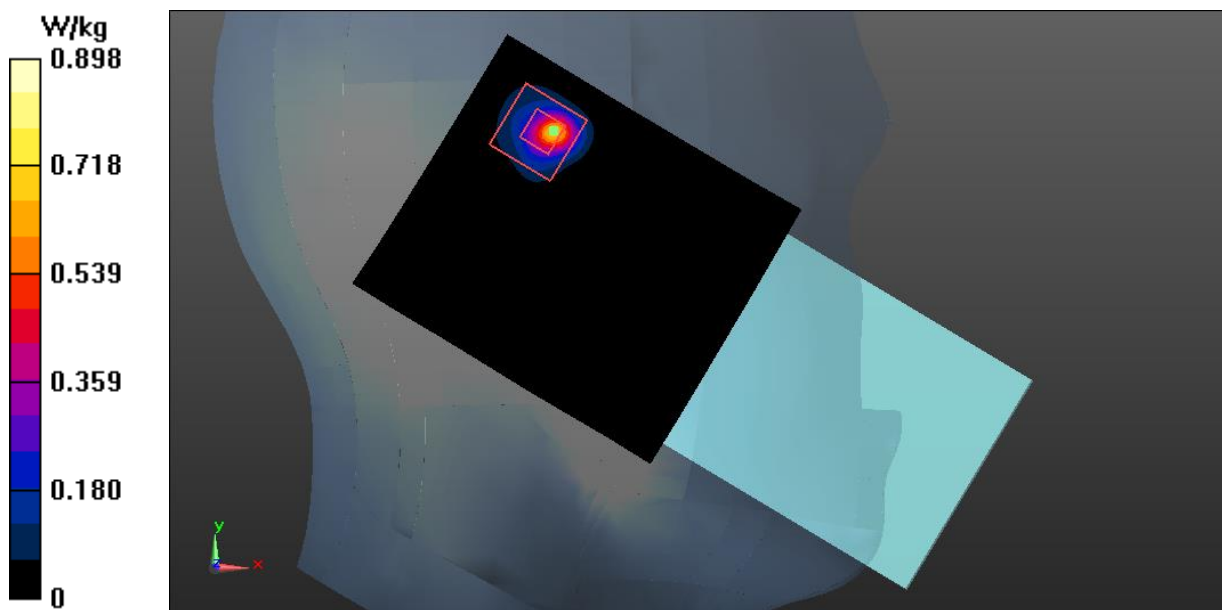
Fig.38 WLAN 5GHz Head
