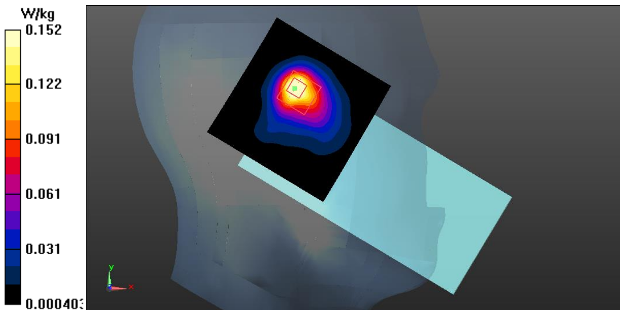
Fig.34 Bluetooth Head
