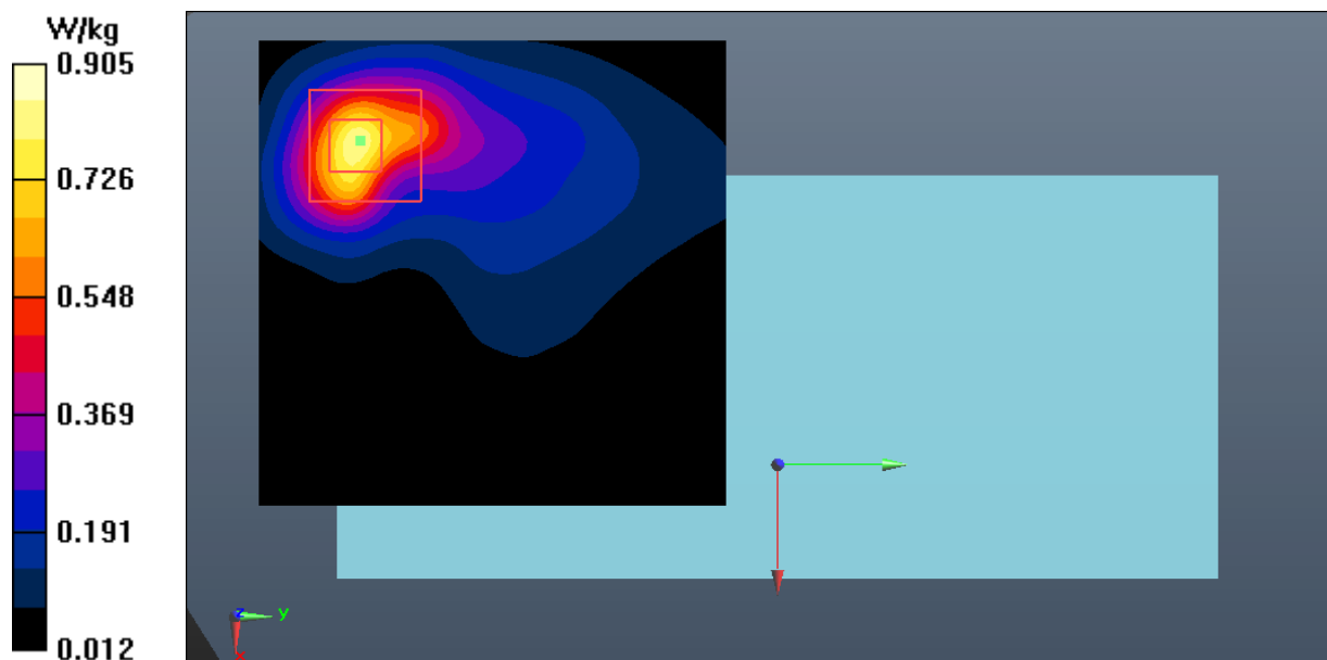
Fig.18 LTE Band 30 Body
