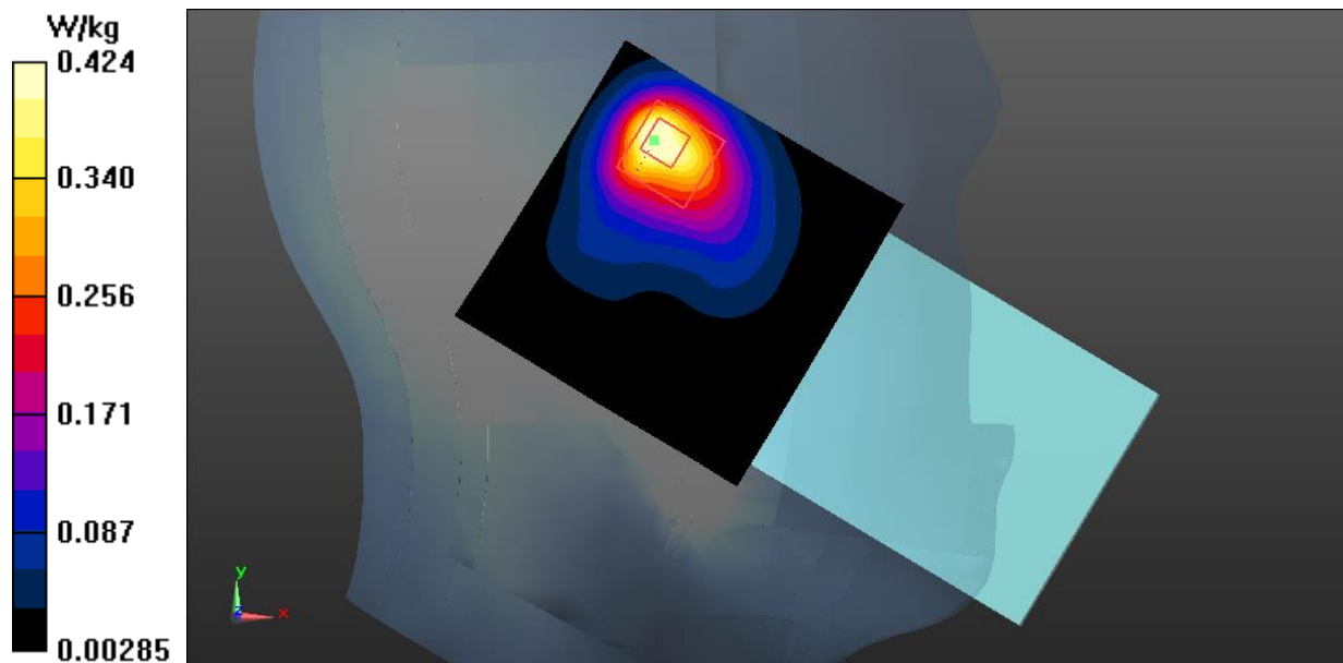
Fig.36 WLAN 2.4GHz Head
