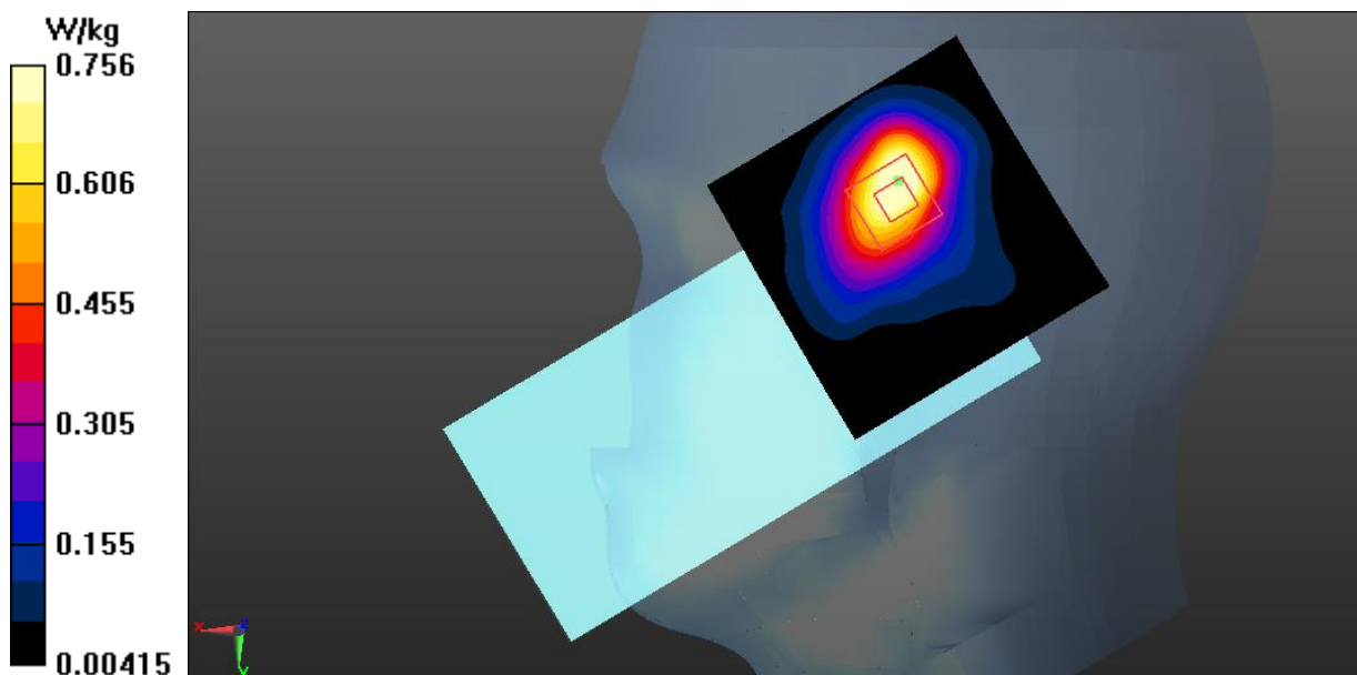
Fig.11 LTE Band 7 Head
