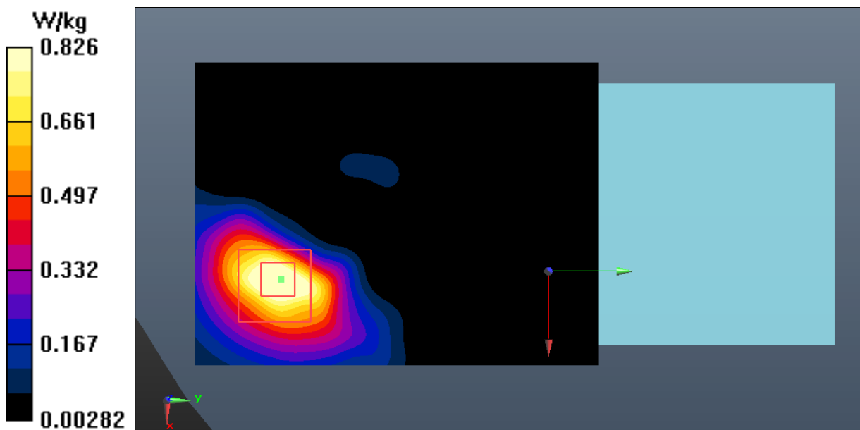
Fig.39 WLAN 5GHz Body
