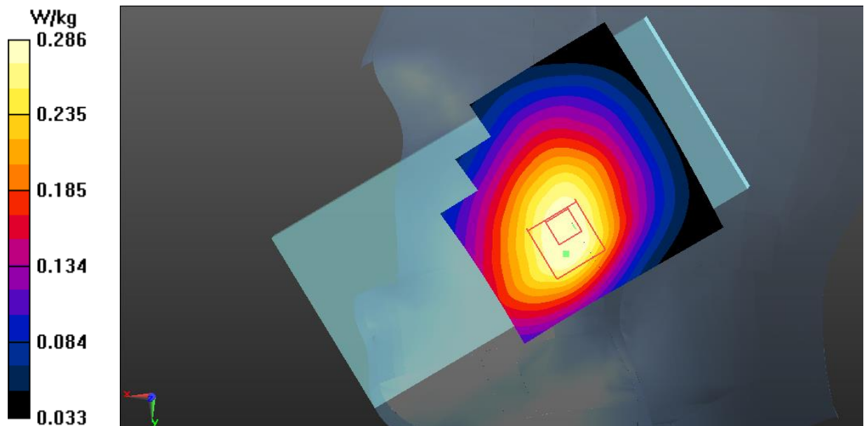
Fig.5 WCDMA Band 5 Head
