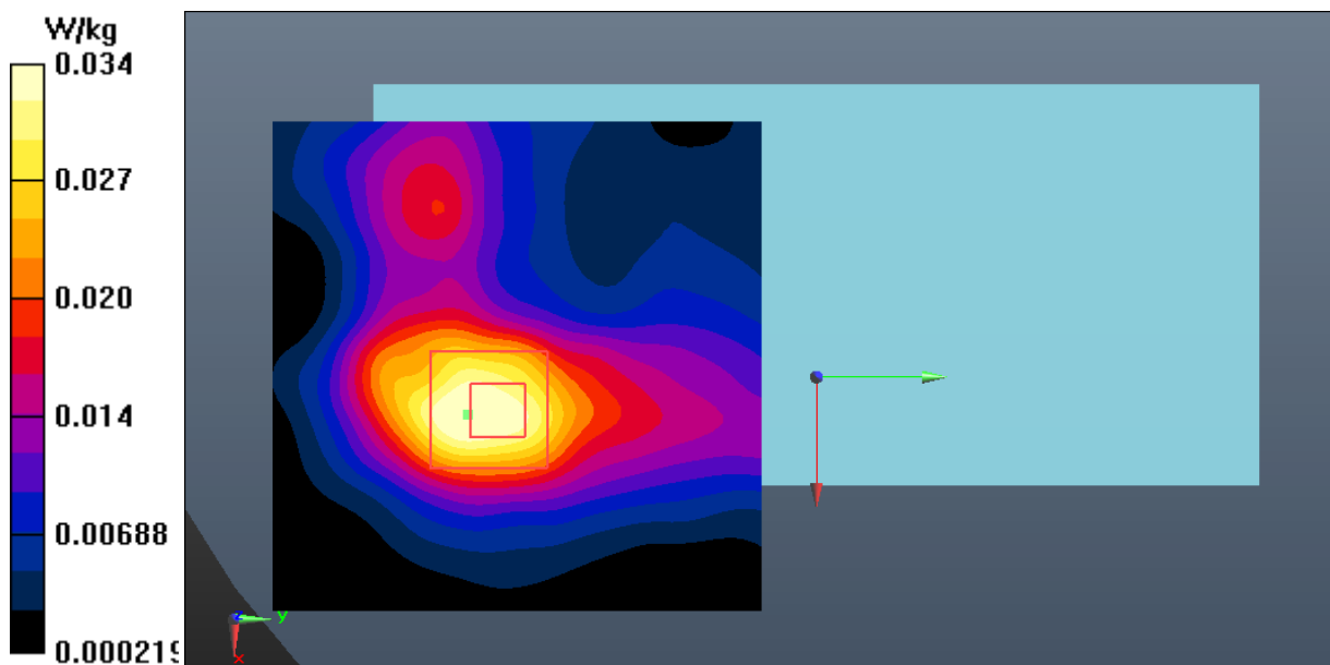
Fig.35 Bluetooth Body
