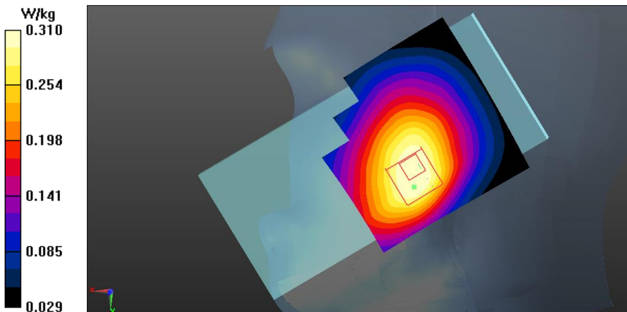
Fig.9 LTE Band 5 Head
