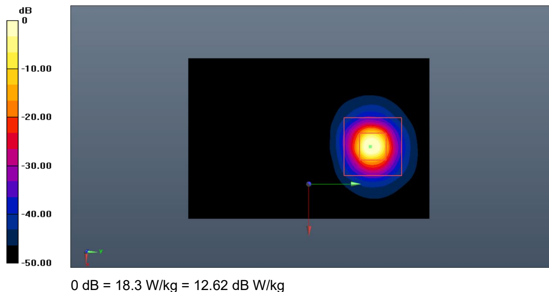
Fig.B.13. Validation 5750MHz 100mW
