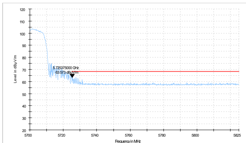
Fig. 8 Band Edges (802.11n-HT20 Ch140, 5700MHz)
