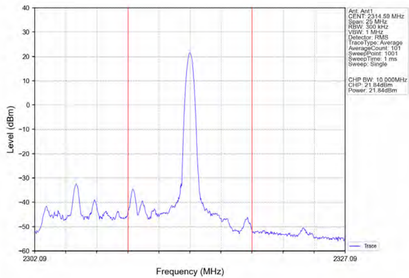
n30_15kHz_SISO_NTNV_10MHz_DFT-s-OFDM_PI/2_BPSK_2310MHz_Edge_1RB_Right_Ant1
