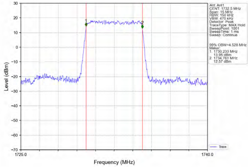
Band4_5MHz_16QAM_MCH_1732.5MHz_RB_25_0_NTNV
