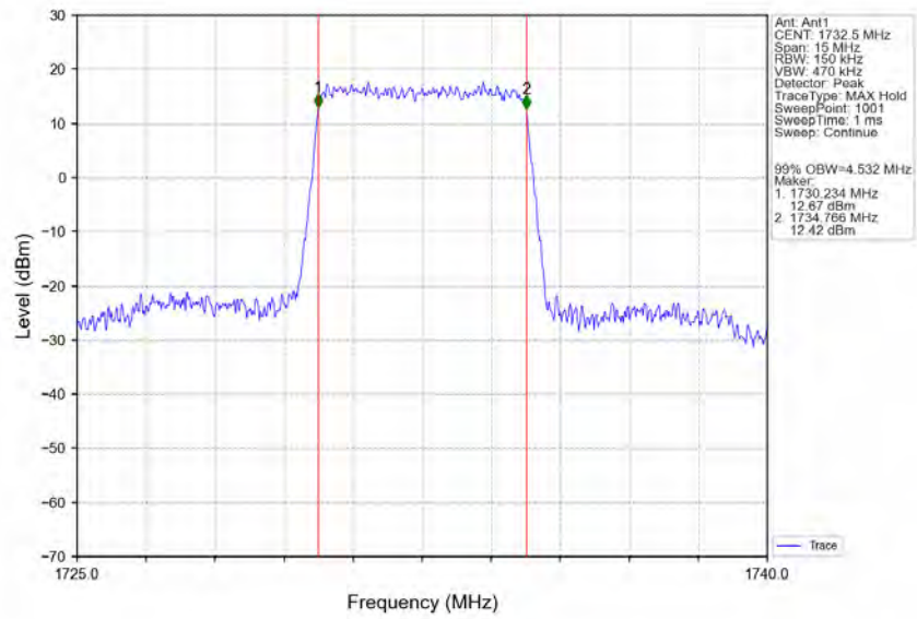
Band4_5MHz_16QAM_MCH_1732.5MHz_RB_25_0_NTNV
