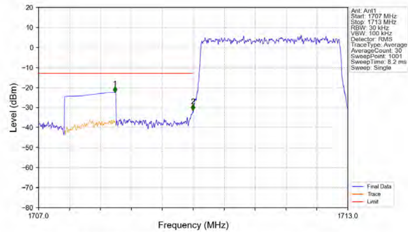
Band4_3MHz_QPSK_LCH_1711.5MHz_RB_15_0_NTNV
