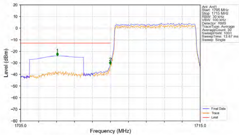
Band4_5MHz_QPSK_LCH_1712.5MHz_RB_25_0_NTNV
