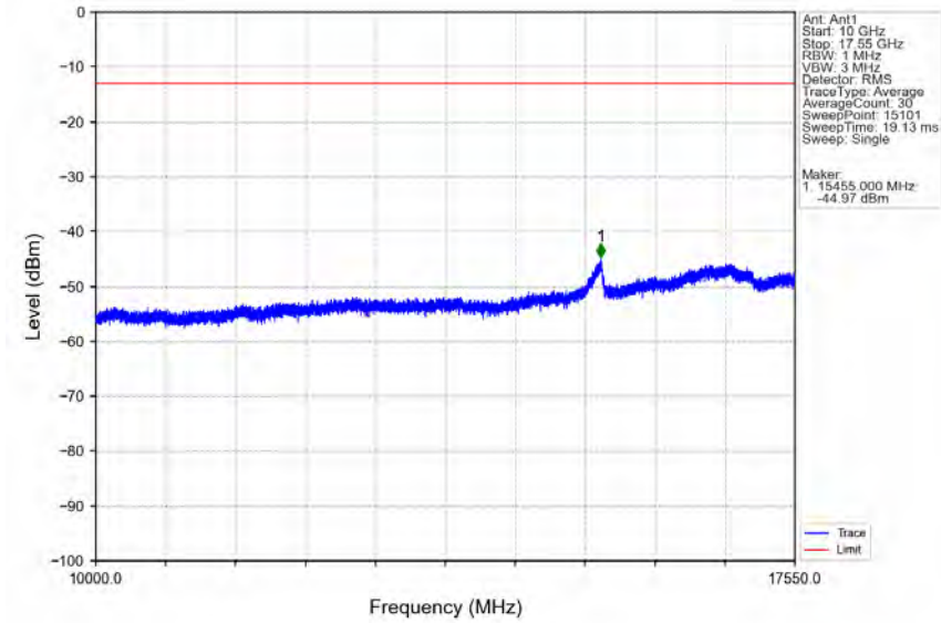
Band4_3MHz_QPSK_LCH_1711.5MHz_RB_15_0_NTNV
