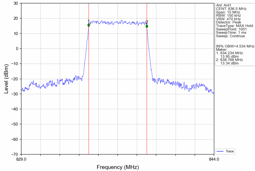
Band5_5MHz_16QAM_MCH_836.5MHz_RB_25_0_NTNV
