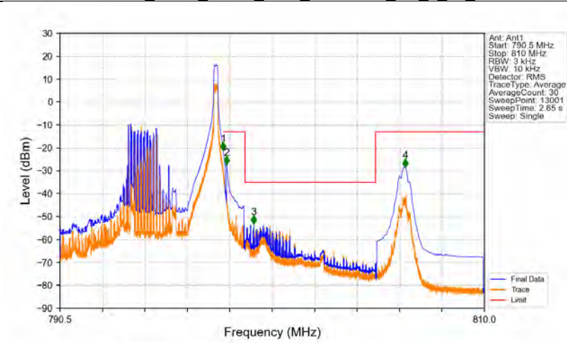
Band14_5MHz_QPSK_HCH_795.5MHz_RB_1_24_NTNV
