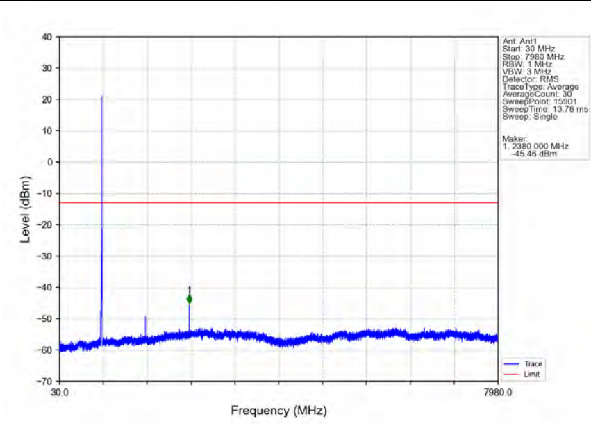
Band14_5MHz_QPSK_HCH_795.5MHz_RB_1_0_NTNV
