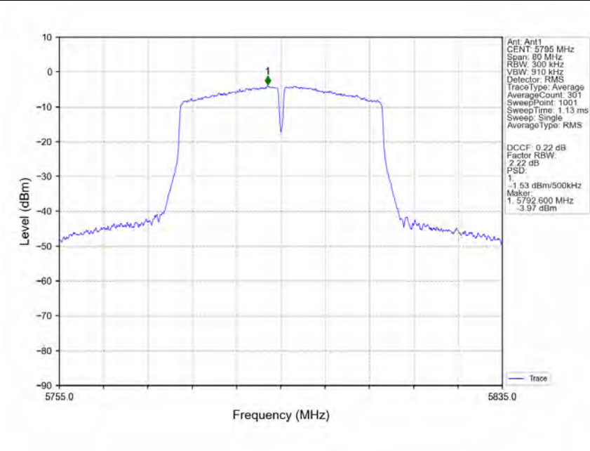
802.11ac(VHT40)_HCH_5795MHz_Ant1_NTNV
