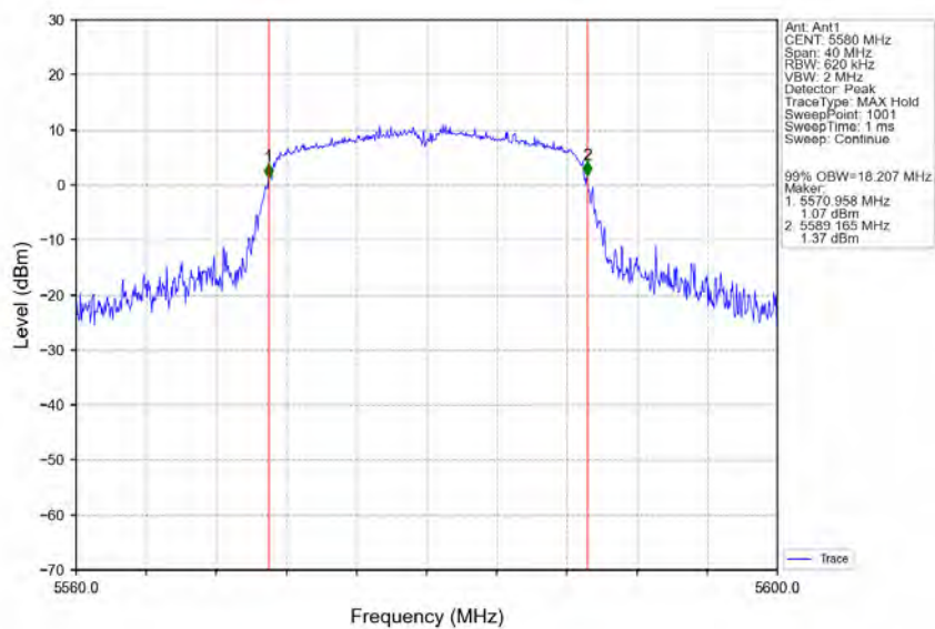
802.11ac(VHT20)_MCH_5580MHz_Ant1_NTNV
