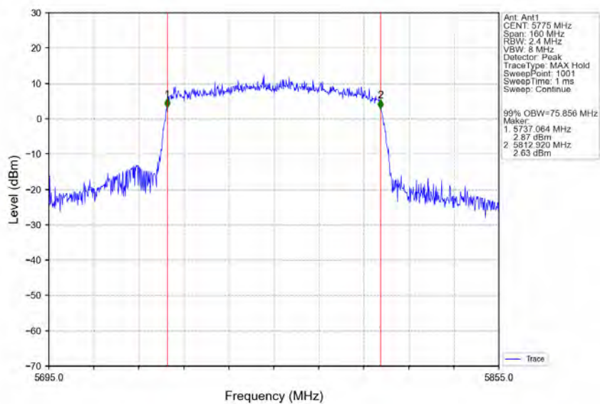
802.11ac(VHT80)_MCH_5775MHz_Ant1_NTNV
