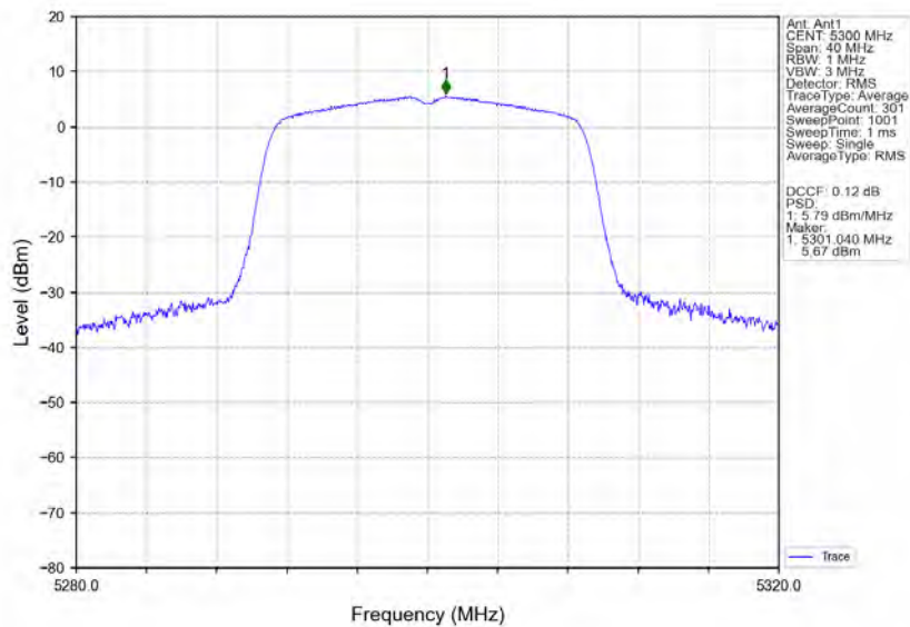
802.11ac(VHT20)_MCH_5300MHz_Ant1_NTNV
