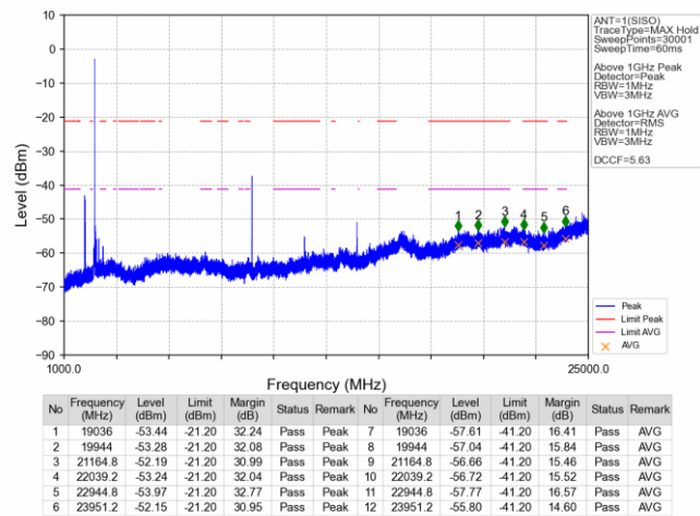
1M_LCH_2402MHz_Ant1_NTNV
