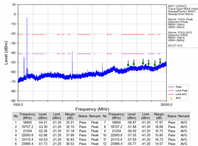
1M_MCH_2440MHz_Ant1_NTNV
