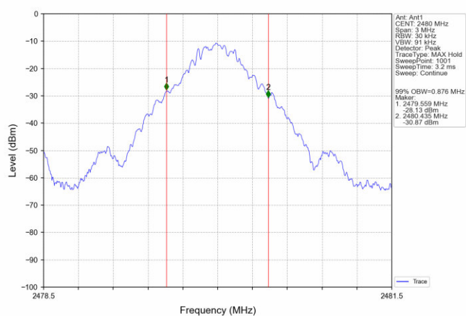
GFSK_DH5_HCH_2480MHz_Ant1_NTNV
