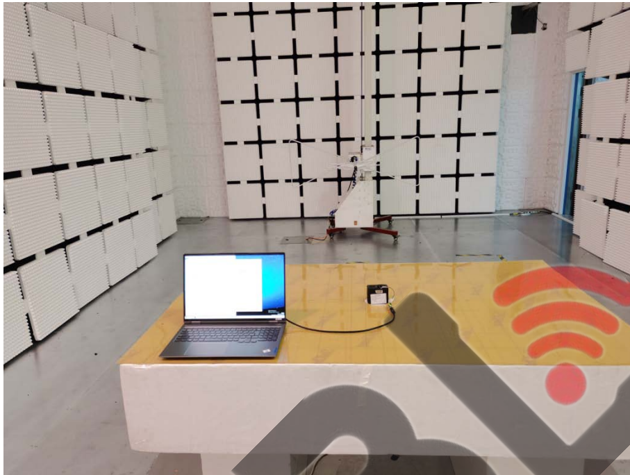
Radiated 30MHz~1GHz
