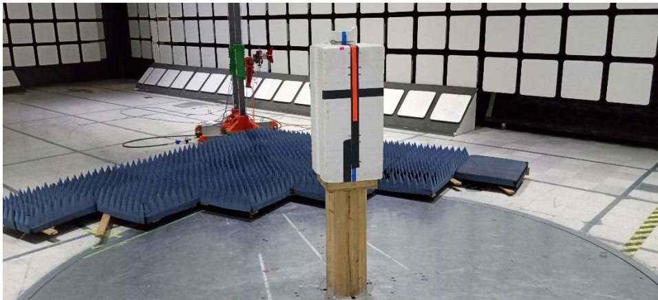
Setup, 1GHz – 18GHz
