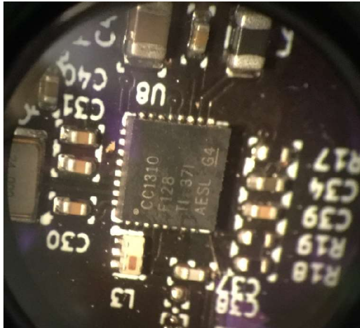
900MHz RF module as part of 2A29A-FBXP
