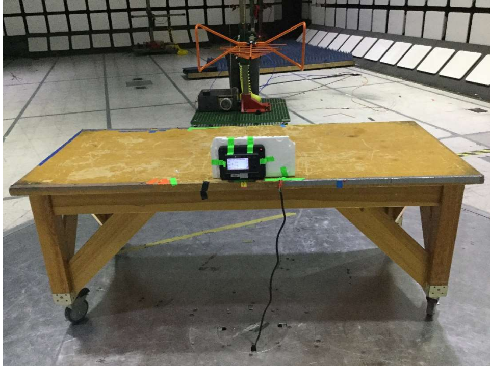
Setup, 30MHz – 1GHz
