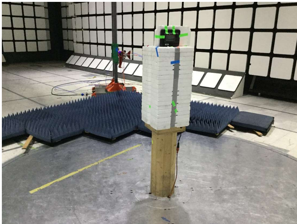
Setup, 1GHz – 18GHz
