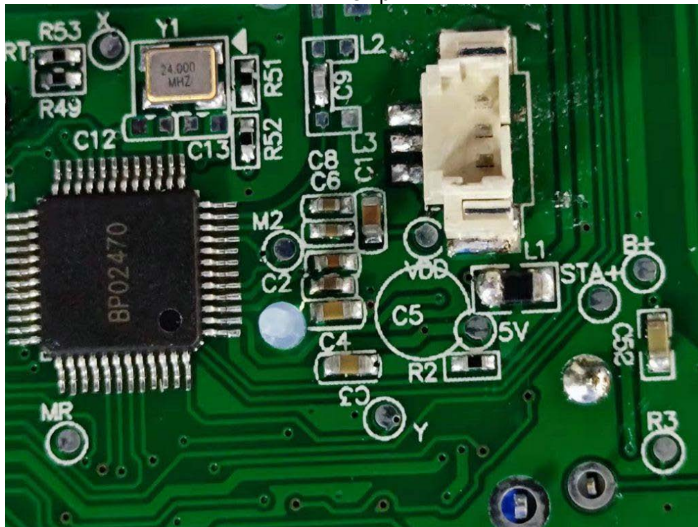
BT Chip
