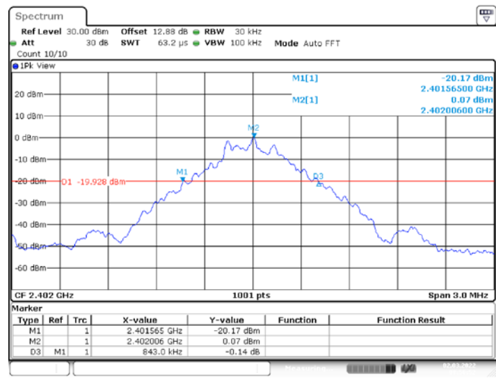
DH1_Ant1_2402MHz
