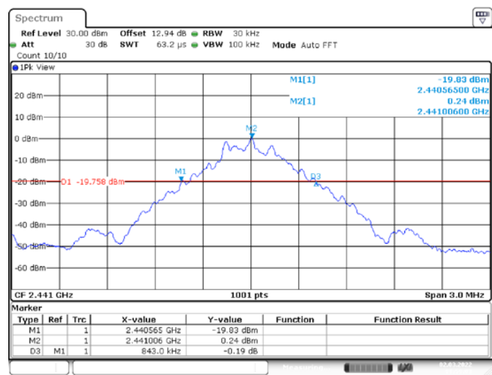
DH1_Ant1_2441MHz
