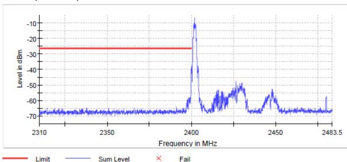
Channel 0 (2402MHz)
