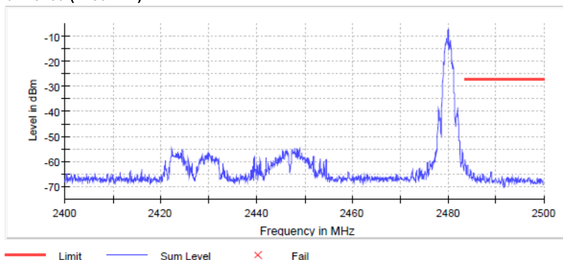
Channel 39 (2480MHz)
