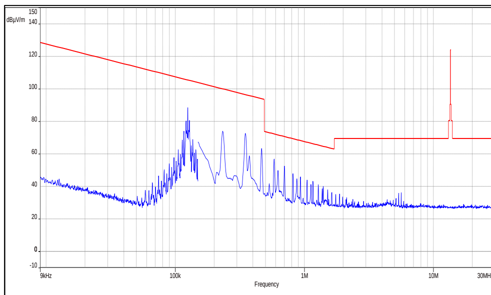
Polarization: Perpendicular
