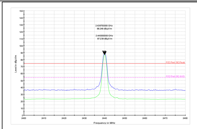
Channel Frequency: 2440MHz Polarization: Vertical
