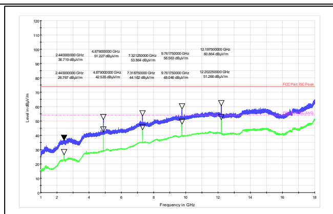
Channel Frequency: 2440MHz Polarization: Vertical
