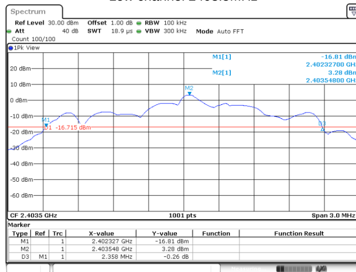
Low channel 2403.5MHz
