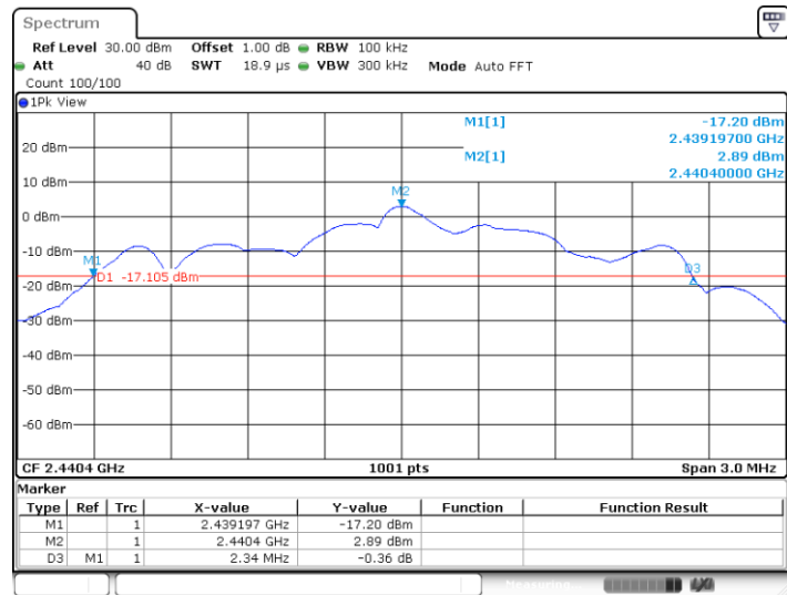
Middle channel 2440.4MHz
