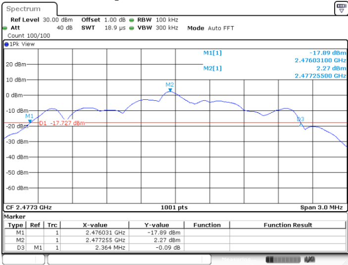
High channel 2477.3MHz
