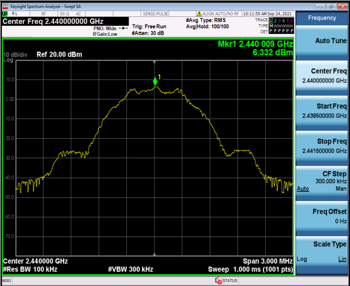
BLE_2440-Reference
