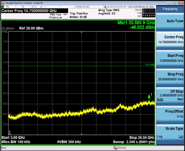
BLE_2440 3000-26500
