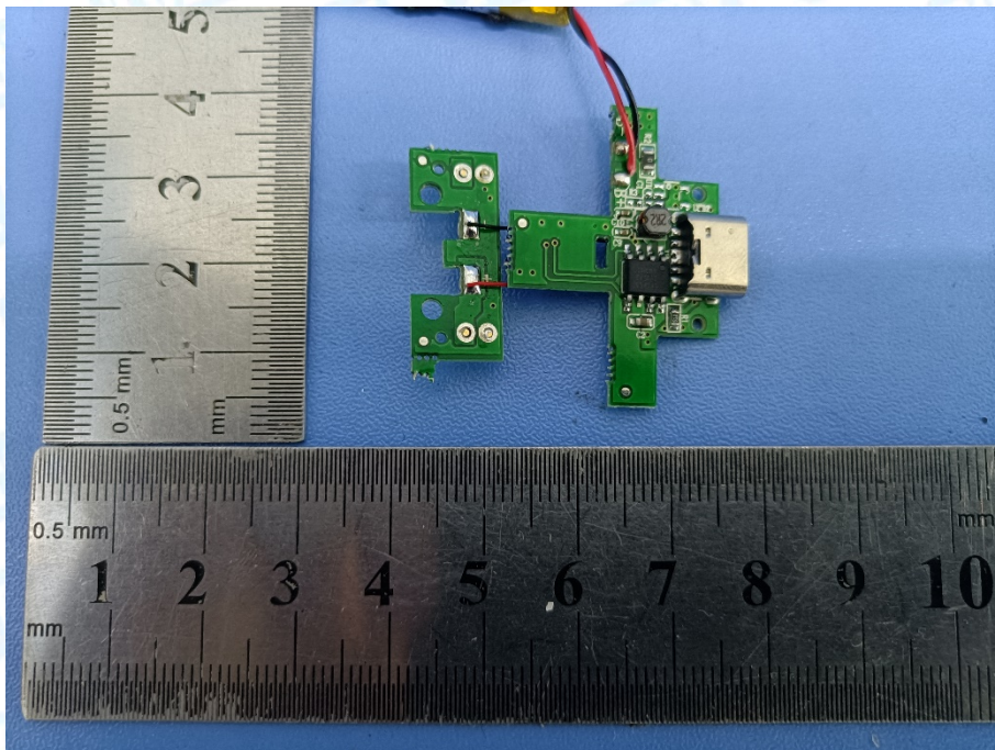
Photo 12 Internal of PCB&Battery
