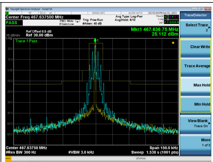
Channel 11: 467.6375MHz
