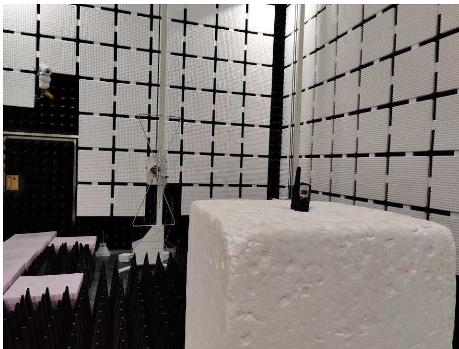
Below 1GHz
