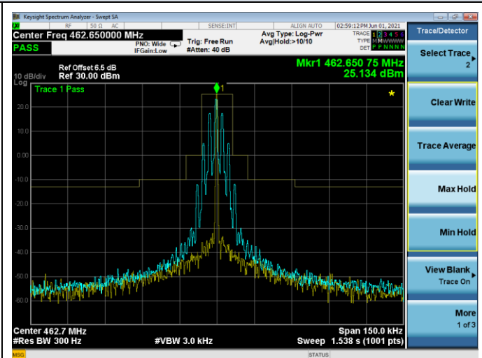
Channel 19: 462.6500MHz
