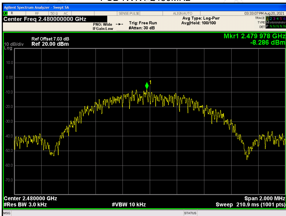
PSD NVNT 2480MHz
