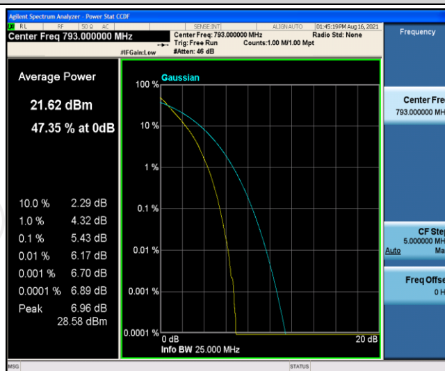
Band14-10MHz-16QAM-23330-1RB#0
