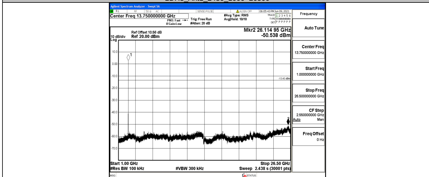
3DH5_Ant1_2402_0~Reference
