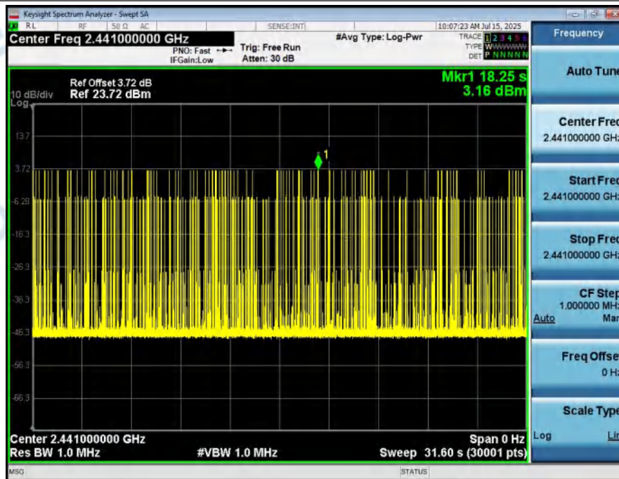
Dwell_Time_(Hopping)_NVNT_ANT1_2-DH5_2441_00_One_Burst_Time
