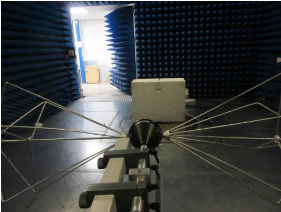
TEST SETUP PHOTO(S) RADIATED EMISSIONS (3MHz>F>300MHz)
