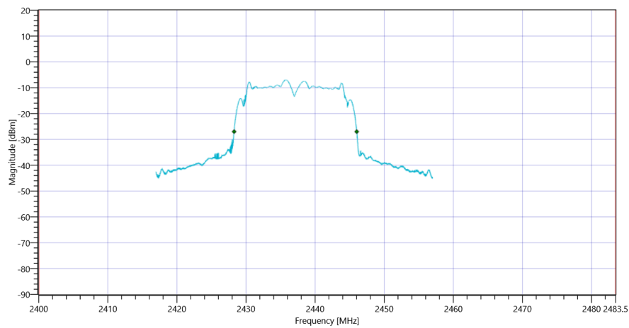
Plot_FCC Part 15.247 Bandwidth 99PCT-20dB ~ WLAN2G4 g-mode_07042021_140623.png
