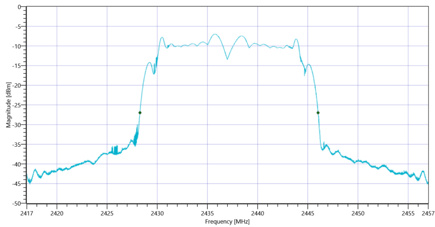
Plot_FCC Part 15.247 Bandwidth 99PCT-20dB ~ WLAN2G4 g-mode_07042021_140616.png
