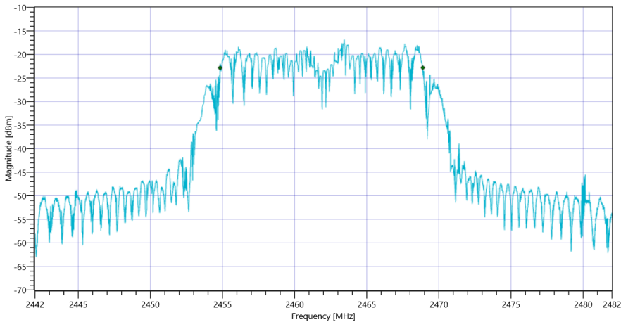
Plot_FCC Part 15.247 Bandwidth 6dB DTS ~ WLAN2G4 g-mode_07042021_141742.png
