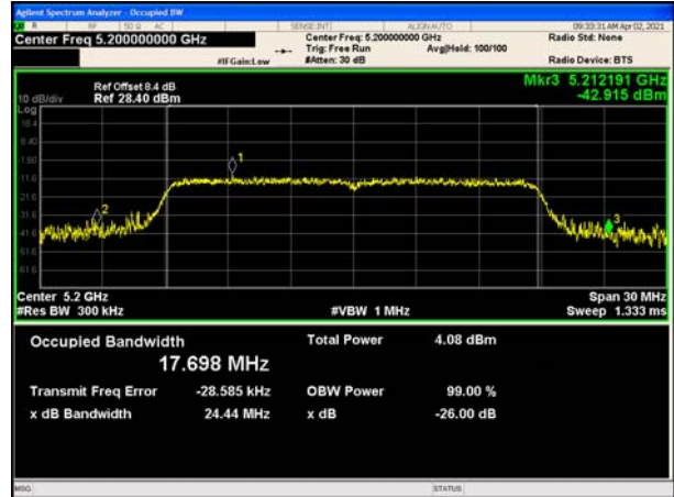
(802.11 n20) 99%Bandwidth plot on channel 40
