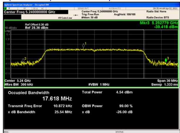
(802.11 n20) 99%Bandwidth plot on channel 48
